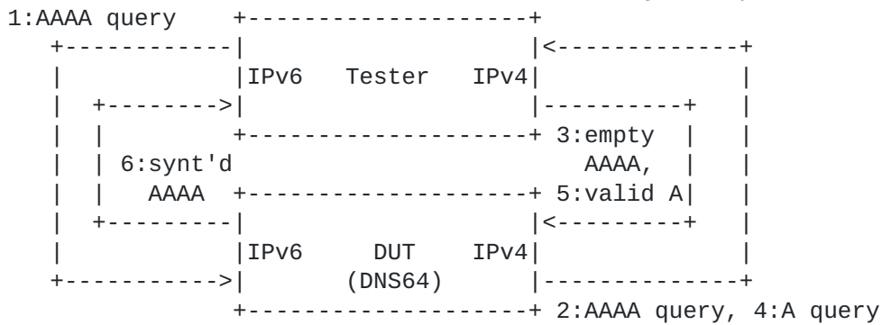
Figure 3. DNS64 test setup
