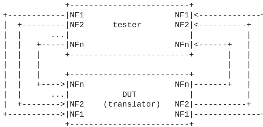
Figure 4. Test setup 3
