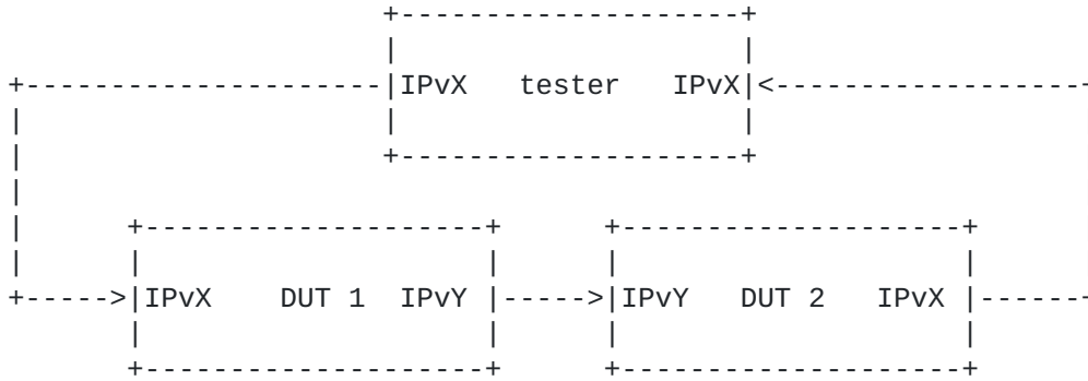
Figure 2. Test setup 2
