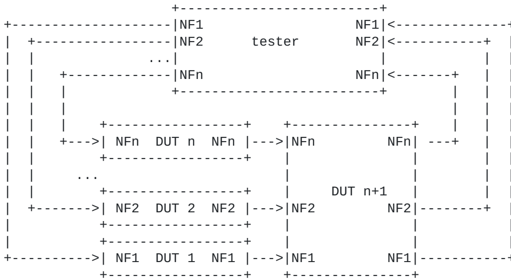
Figure 5. Test setup 4
