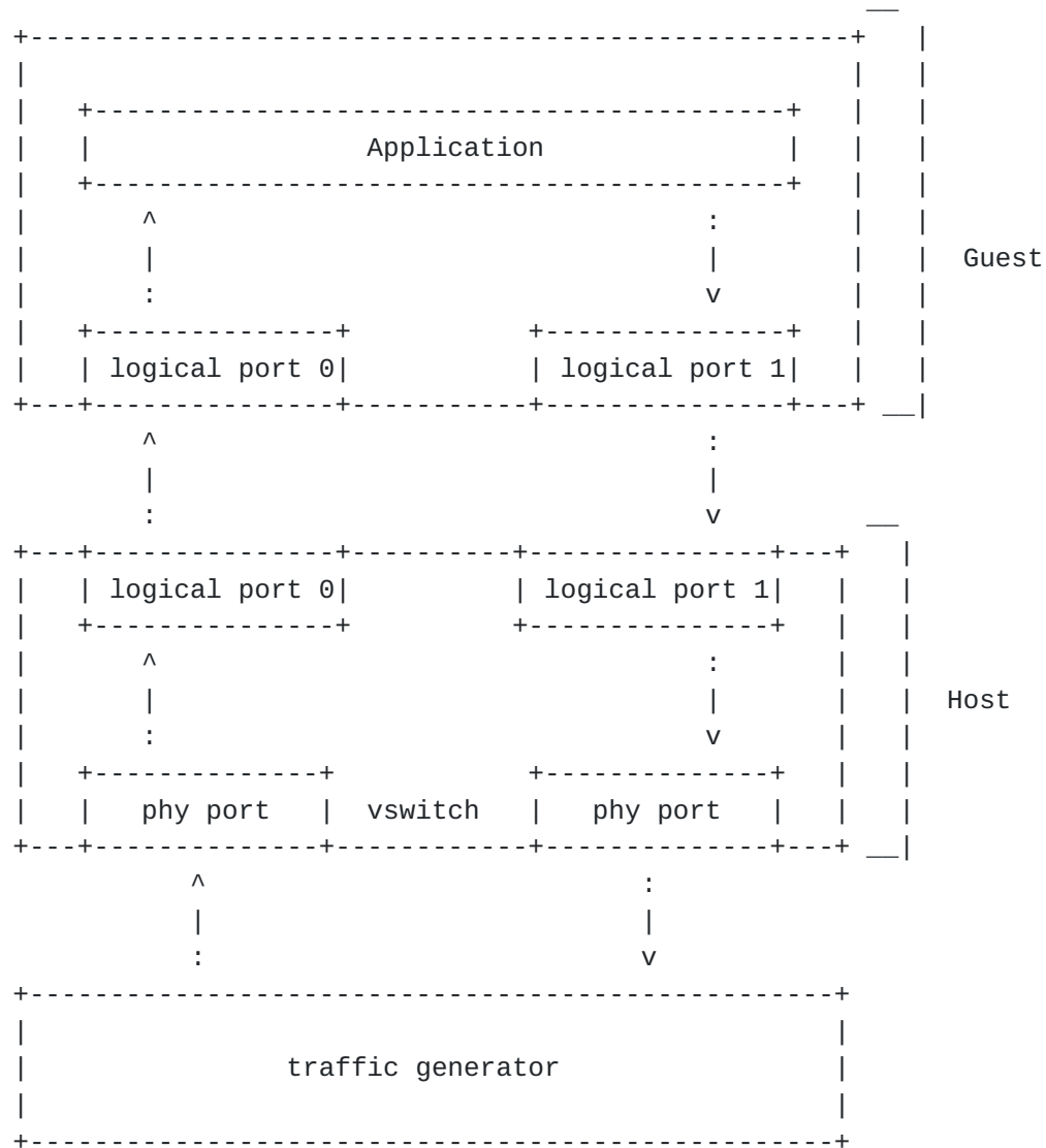
Figure 4 Physical port to virtual switch to VNF to virtual switch to physical port
