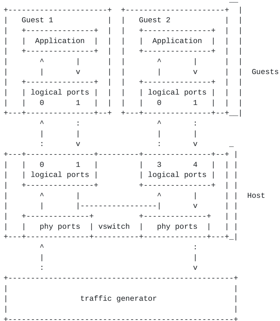
Figure 5 Physical port to virtual switch to VNF to virtual switch to VNF to virtual switch to physical port
