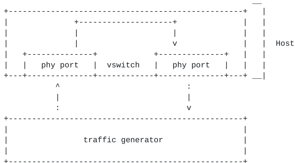
Figure 3 Physical port to virtual switch to physical port
