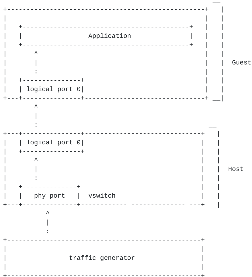
Figure 6 Physical port to virtual switch to VNF
