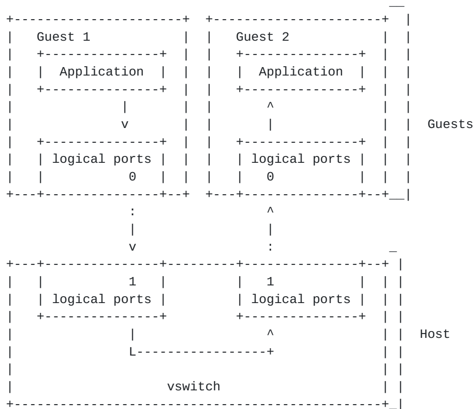
Figure 8 VNF to virtual switch to VNF
