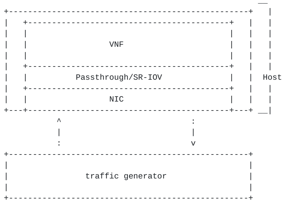
Figure 2 Benchmark VNF forwarding capability
