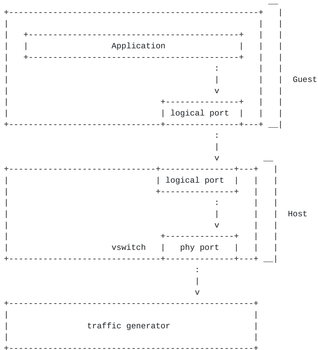
Figure 7 VNF to virtual switch to physical port
