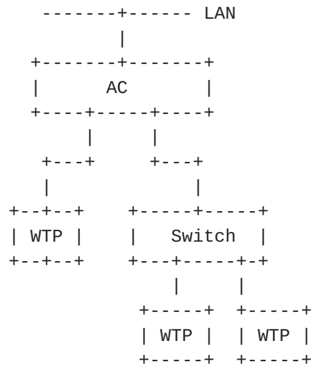
Figure 4: Switched Connections
