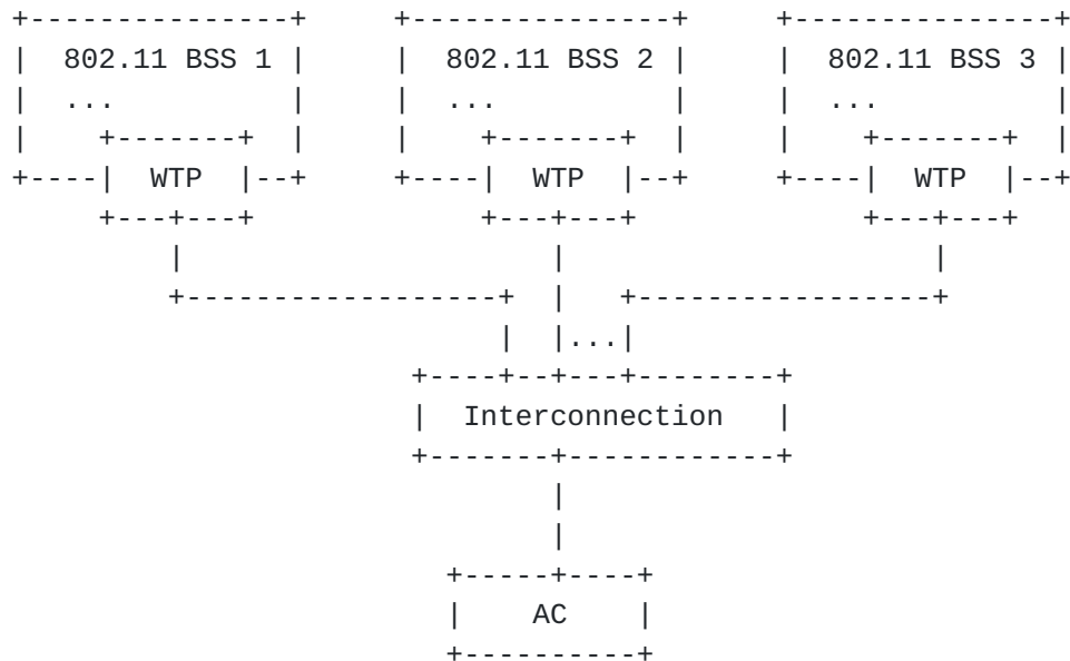
Figure 2: Centralized WLAN Architecture Diagram
