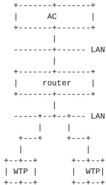
Figure 5: Routed Connections
