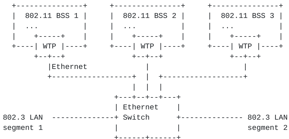
Figure 1: Example of Autonomous WLAN Architecture
