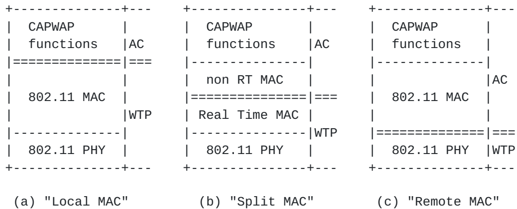
Figure 6: Three Architectural Variants within Centralized WLAN Architecture Family
