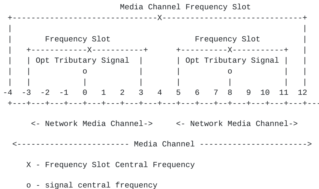
Figure 7: Example of Media Channel / Network Media Channels and associated frequency slots
