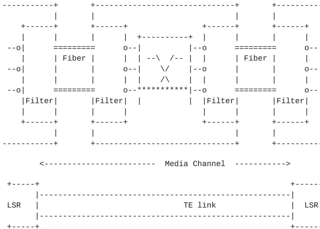
Figure 10: Extended Media Channel / TE Link / FA
