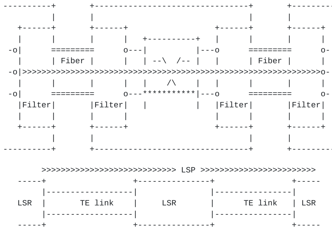
Figure 11: Flex-grid LSP representing a media channel that starts at the filter of the outgoing interface of the ingress LSR and ends at the filter of the incoming interface of the egress LSR
