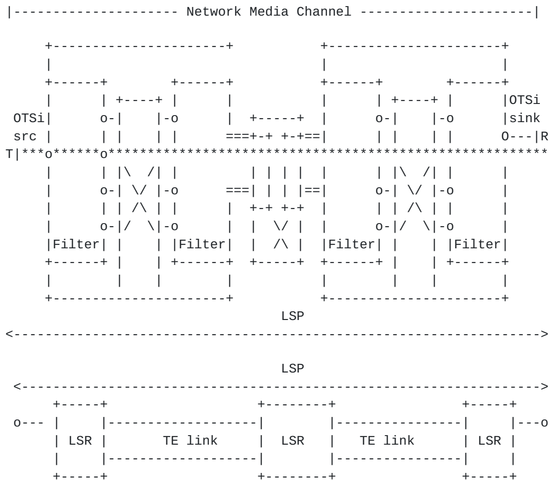
Figure 12: LSP Representing a Network Media Channel (OTSi Trail)
