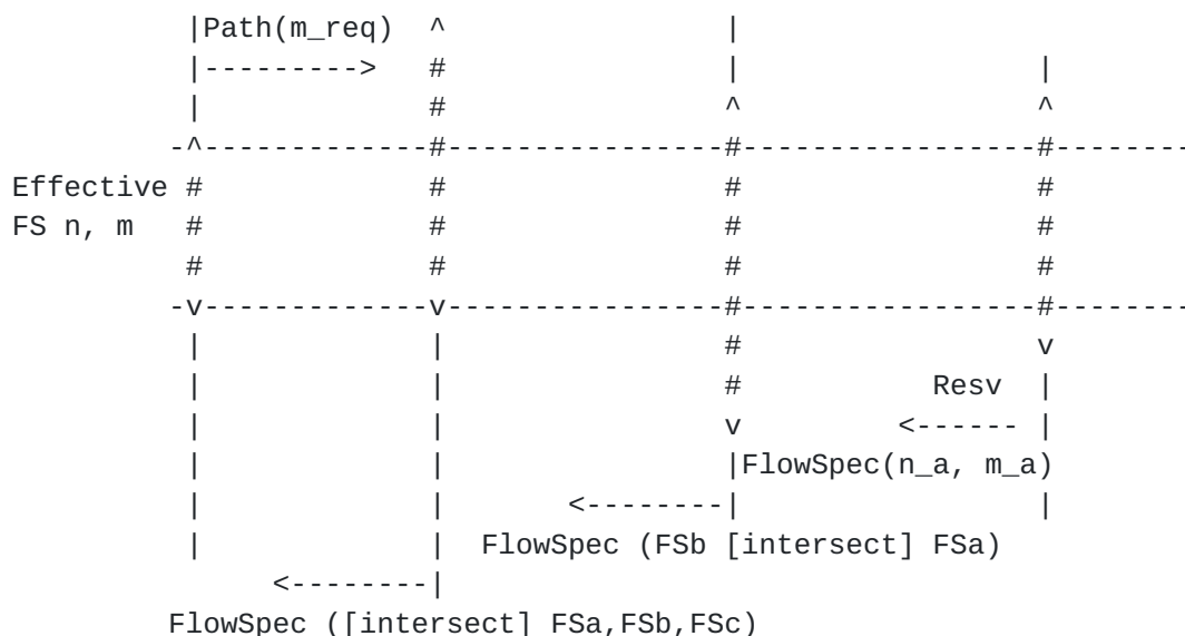
Figure 16: Distributed Allocation with Different m and Different n
