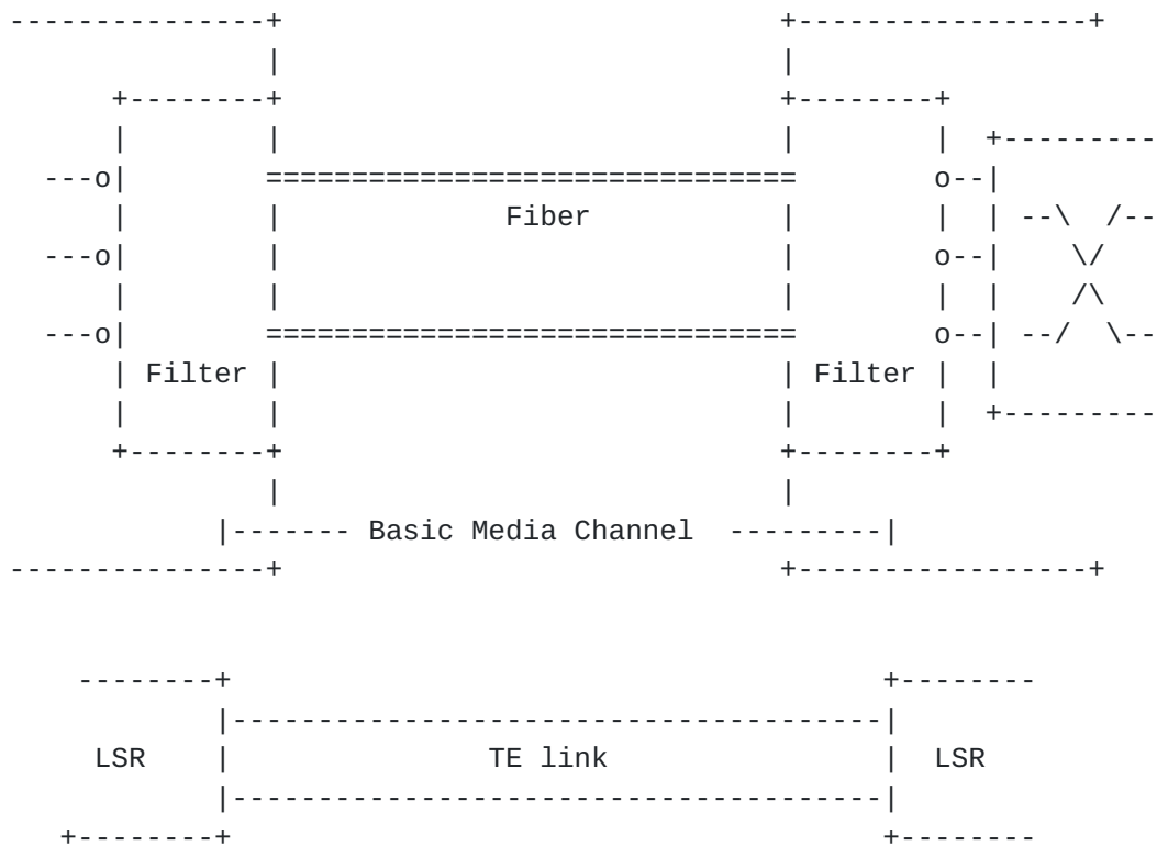
Figure 8: (Basic) Media Channel and TE Link
