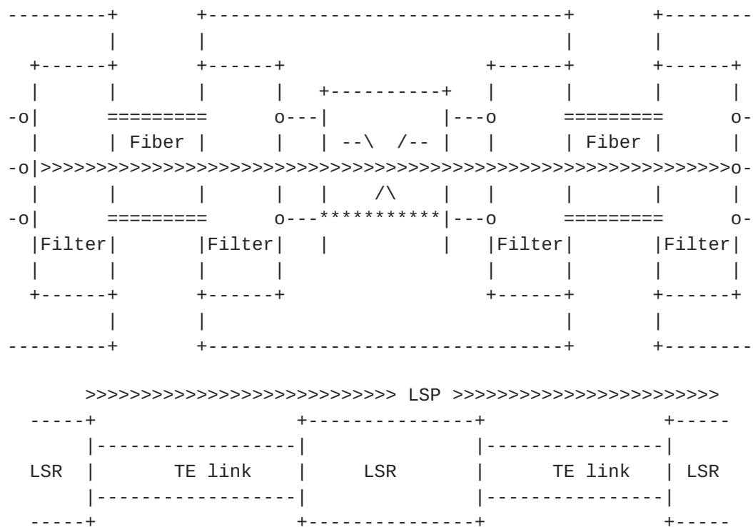
Figure 11: Flex-grid LSP Representing a Media Channel that Starts at the Filter of the Outgoing Interface of the Ingress LSR and ends at the Filter of the Incoming Interface of the Egress LSR
