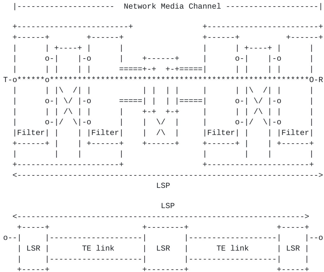
Figure 13: LSP Representing a Network Media Channel (OTSi Network Connection)
