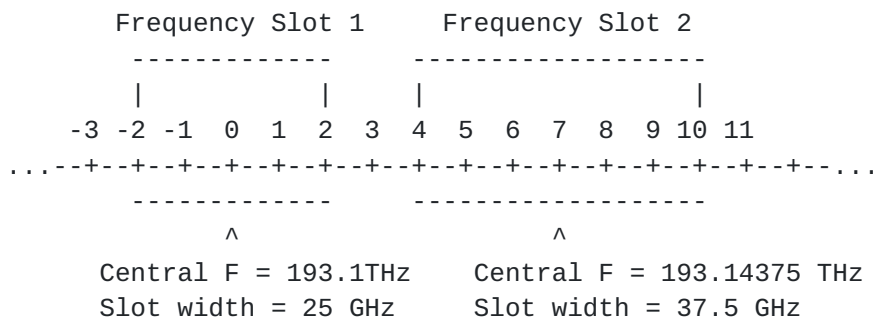
Figure 3: Example Frequency Slots
