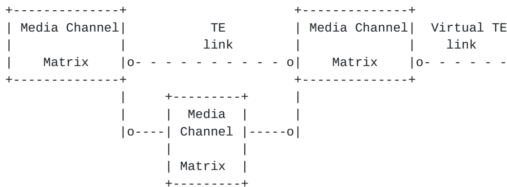
Figure 14: Topology View with TE Link / FA
