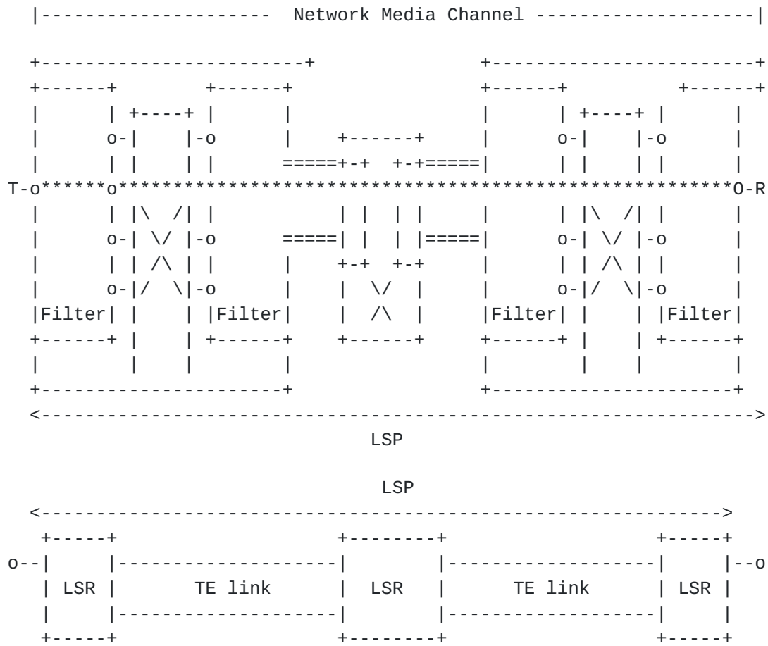
Figure 13: LSP Representing a Network Media Channel (OTSi Network Connection)
