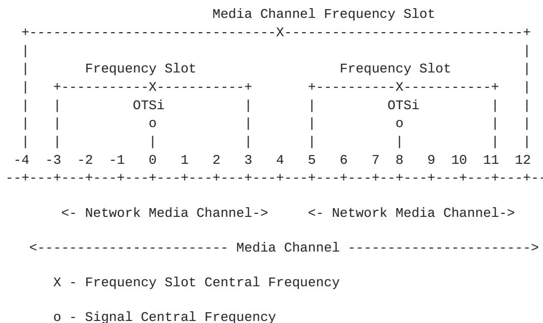
Figure 5: Example of Media Channel / Network Media Channels and Associated Frequency Slots
