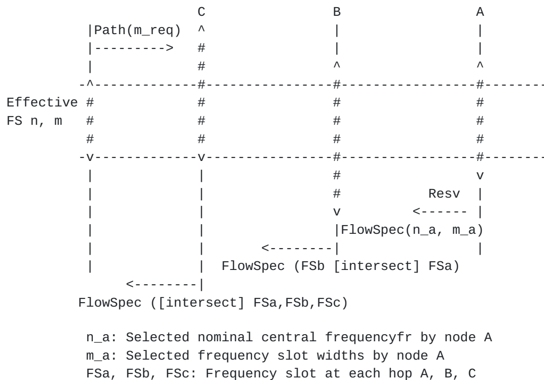
Figure 16: Distributed Allocation with Different m and Different n
