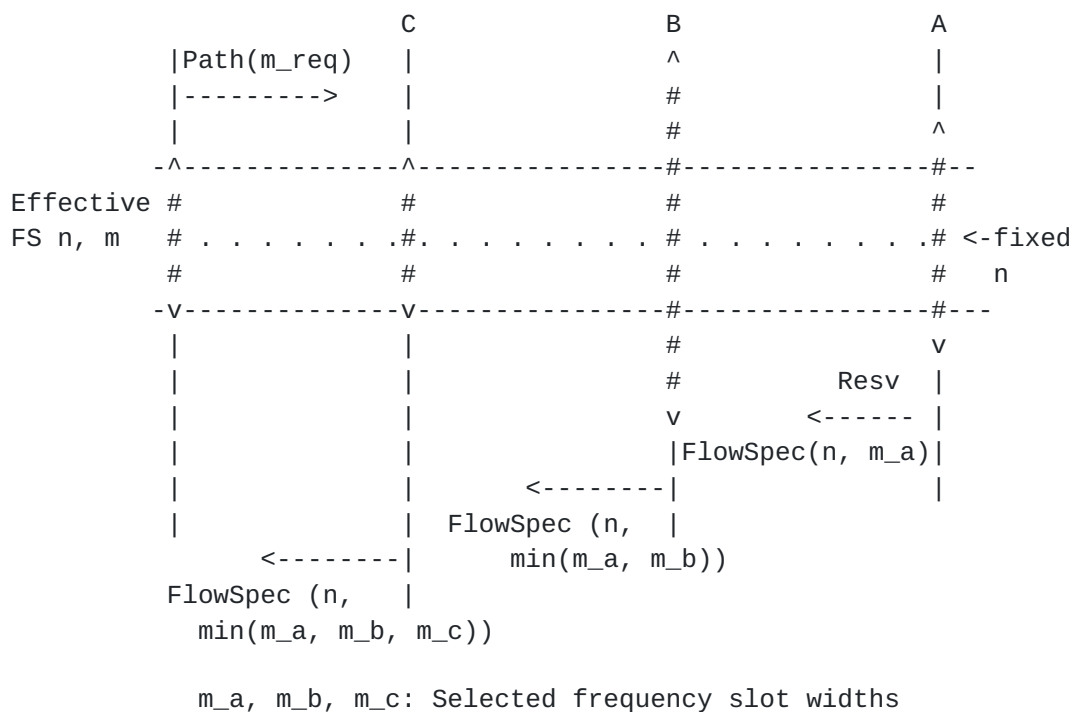
Figure 15: Distributed Allocation with Different m and Same n
