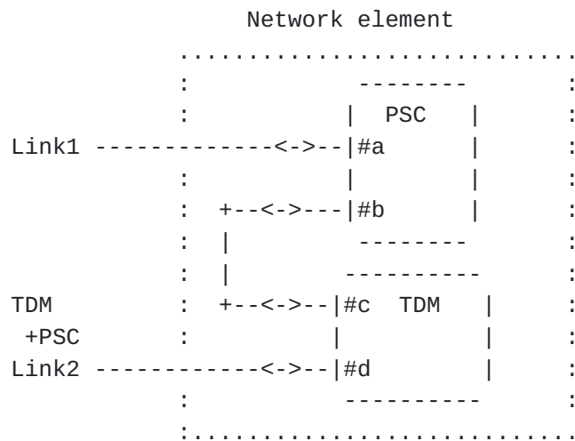
Figure 1. Hybrid node.
