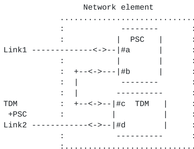
Figure 1. Hybrid node.
