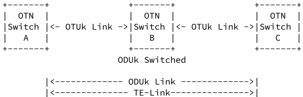
Figure 2: Multiple hop TE-Link
