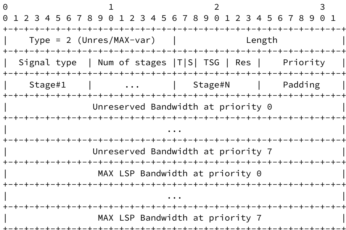
Figure 4: Bandwidth TLV - Type 2 -
