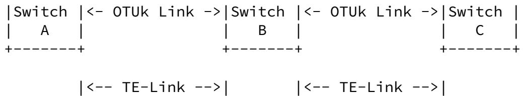
Figure 1: ODUk TE-Links
