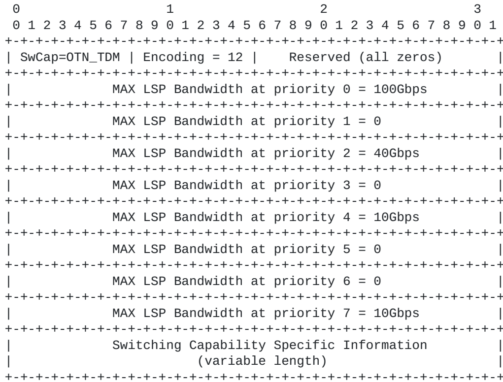
Figure 7: Example 1 - MAX LSP Bandwidth fields in the ISCD at T2
