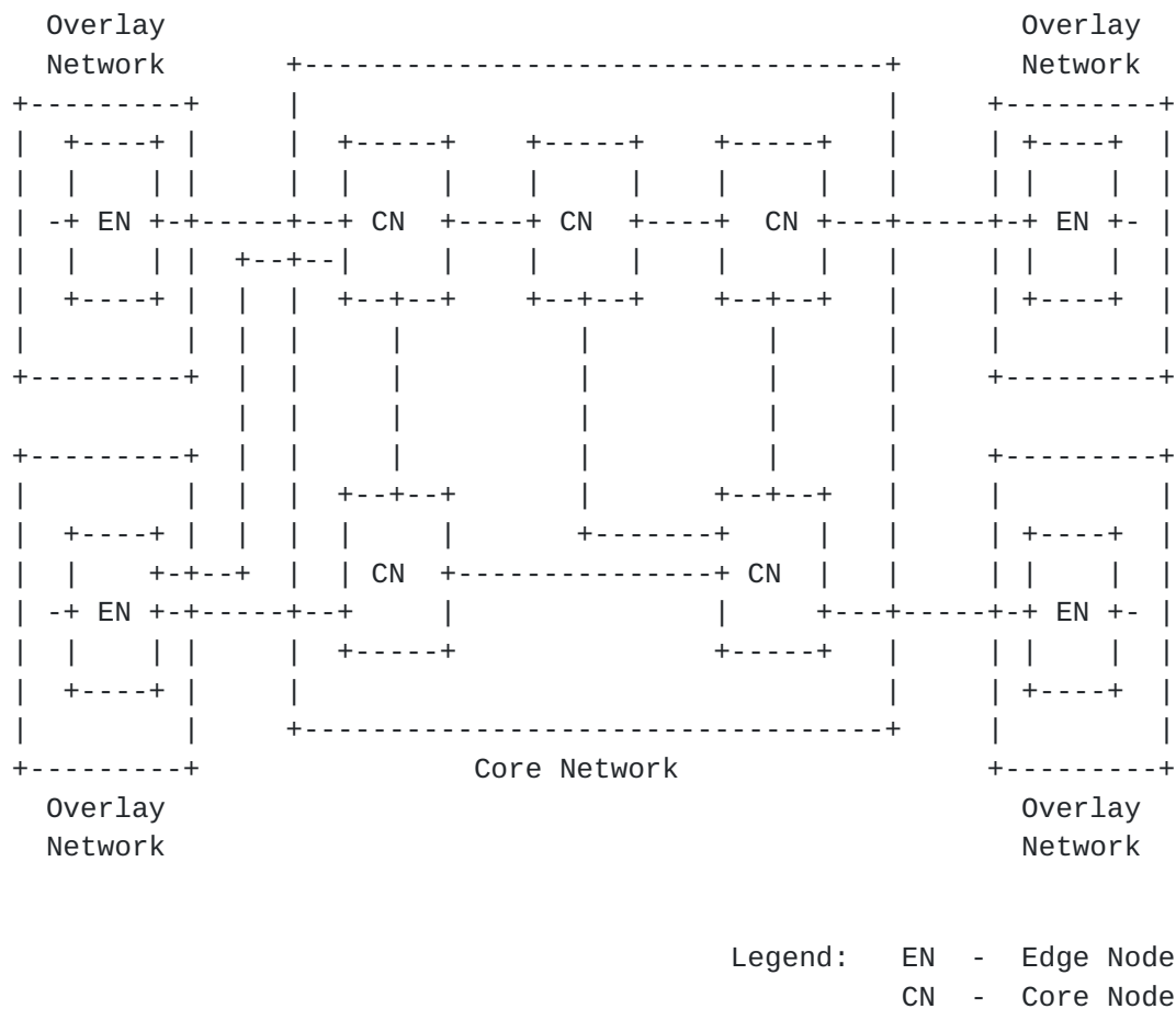
Figure 1: Overlay Reference Model
