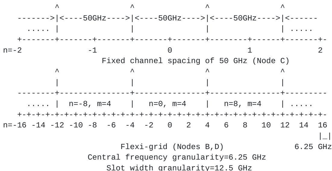
Figure 2: Representation of fixed channel spacing and flexi-grid spectrum slot
