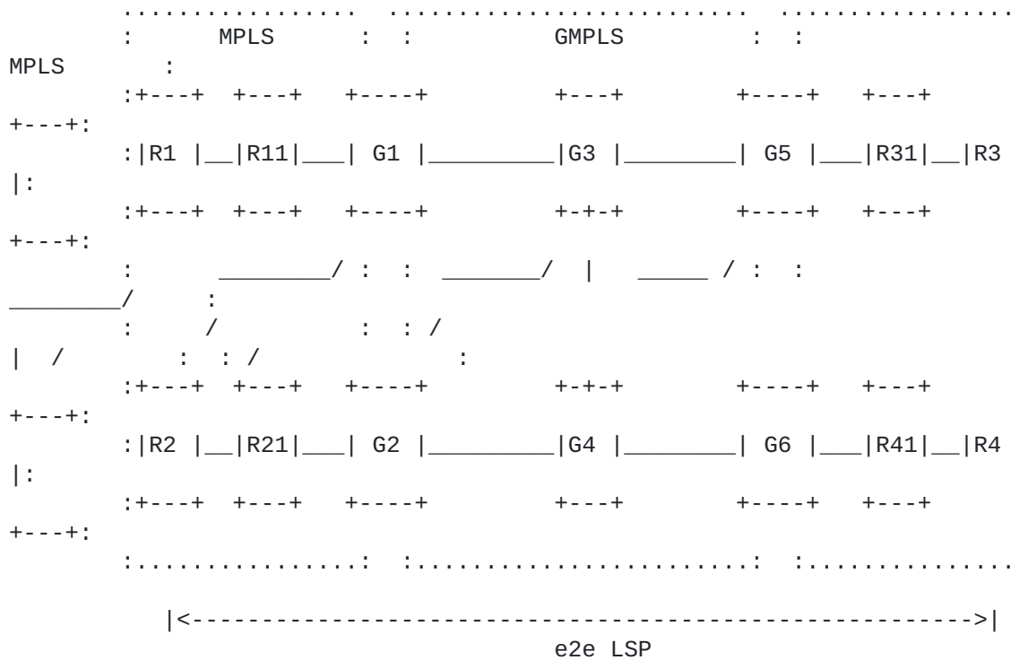
Figure 1 Example of the island model for MPLS-GMPLS-MPLS interworking.
