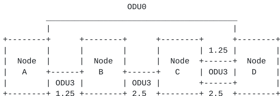
Figure 5: TSG in signaling
