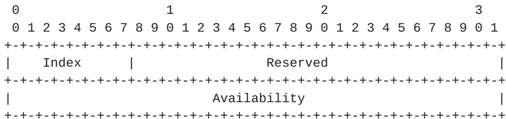
Figure 1: Availability TLV
