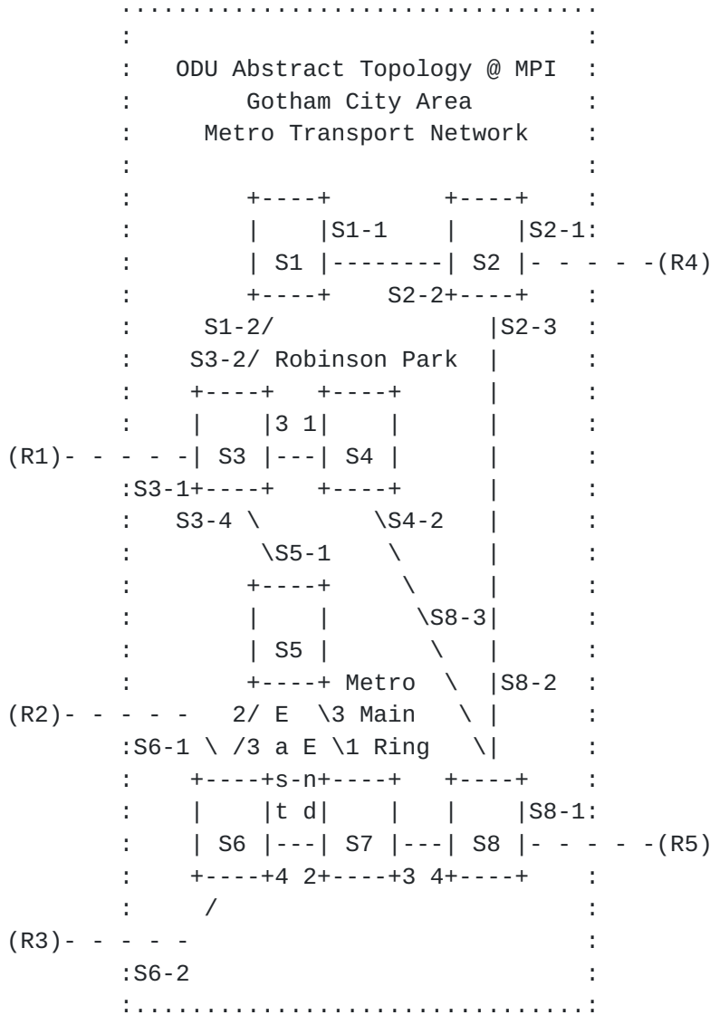
Figure 3 Abstract Topology exposed at MPI1 (MPI1 ODU Topology)
