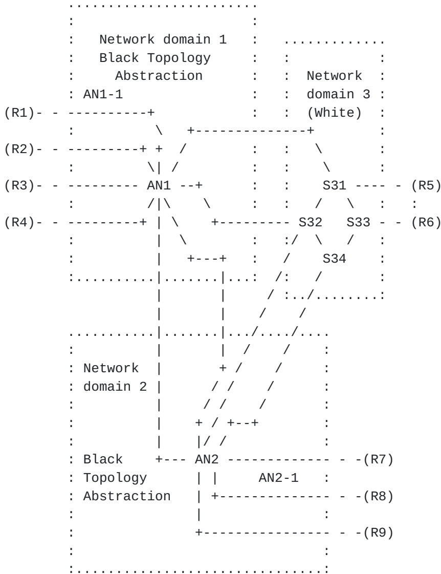
Figure 6 - Multi-domain Abstract Topology controlled by an MDSC
