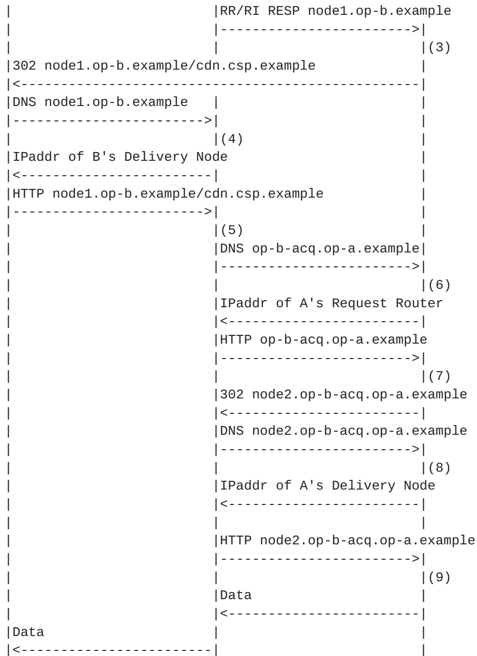
Figure 4: Message Flow for Recursive HTTP Redirection
