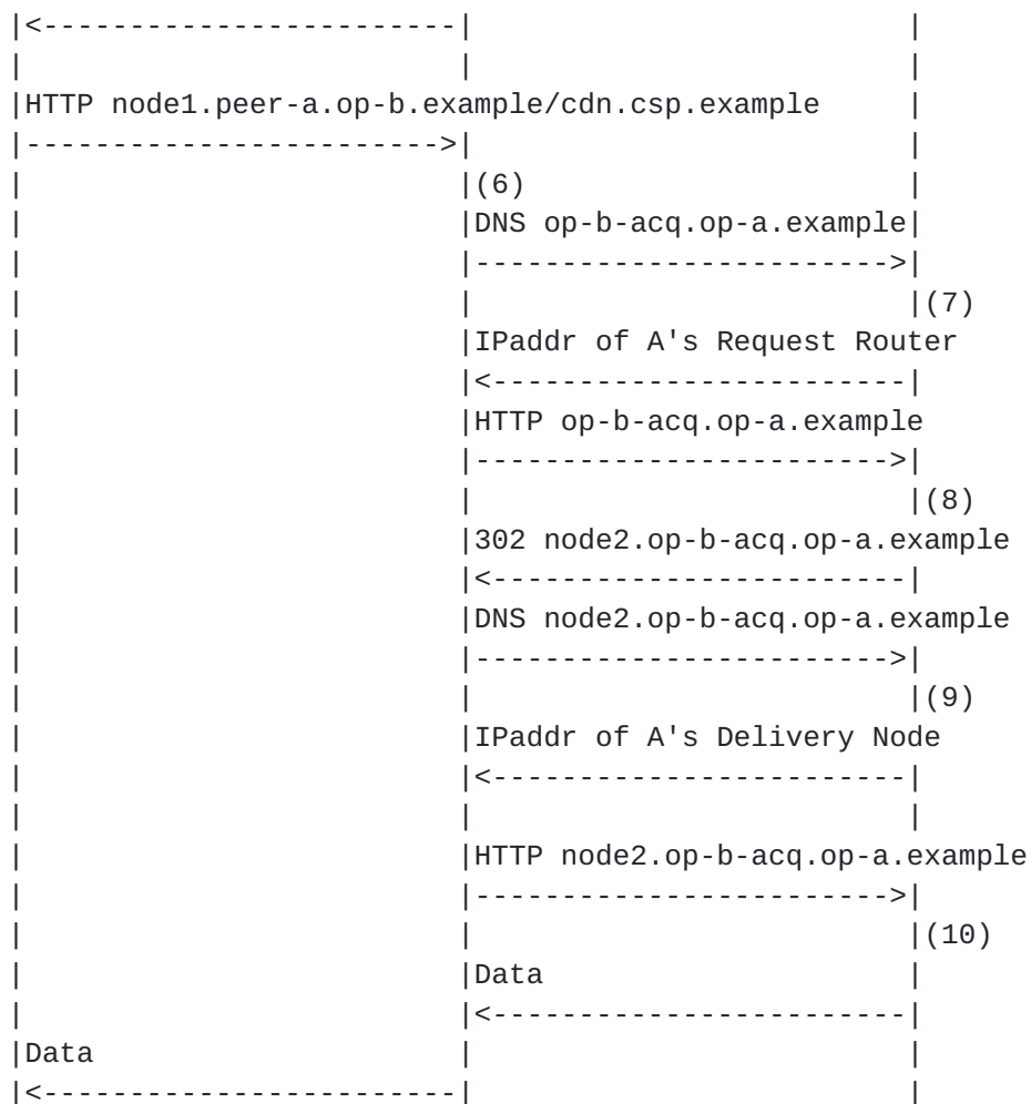
Figure 3: Message Flow for Iterative HTTP Redirection
