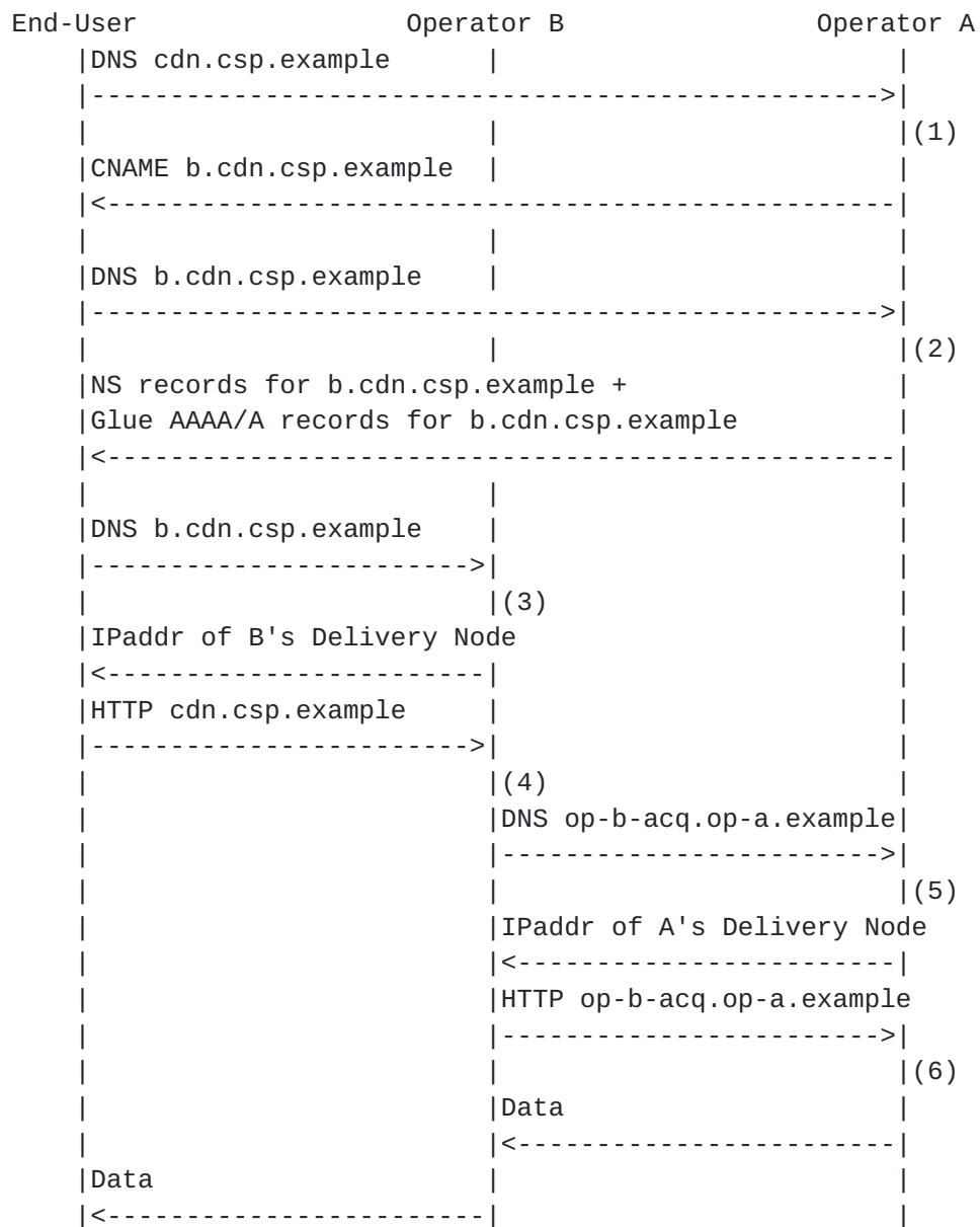
Figure 5: Message Flow for DNS-based Redirection
