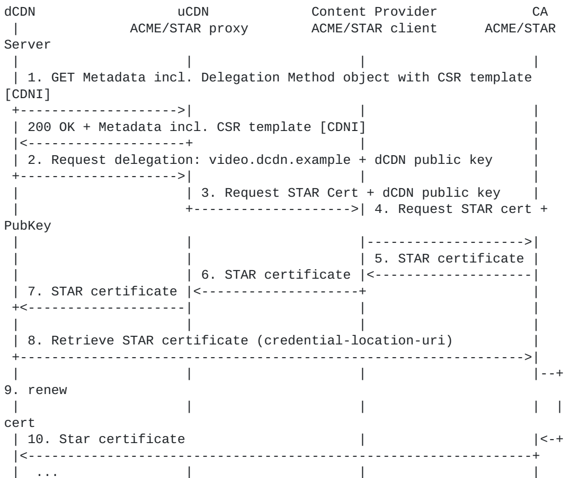
Figure 1: Example call-flow of STAR delegation in CDNI showing 2 levels of delegation
