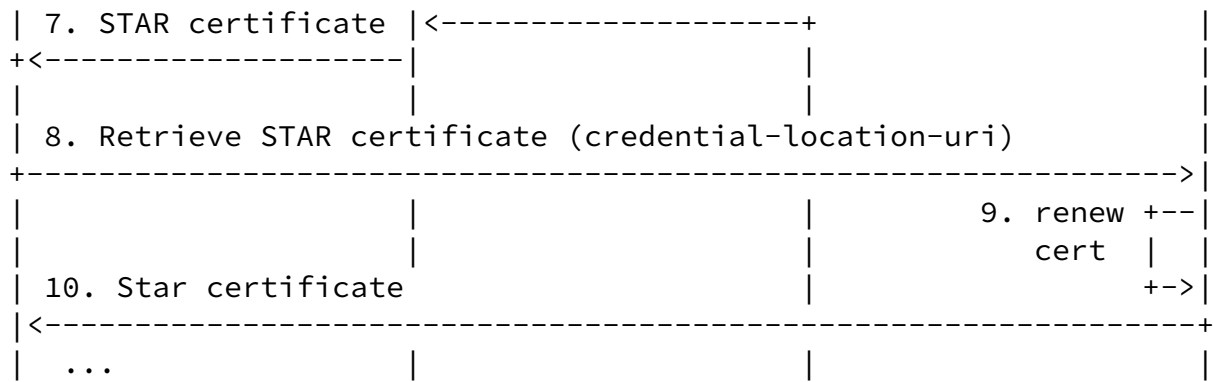
Figure 1: Example call-flow of STAR delegation in CDNI showing 2 levels of delegation
