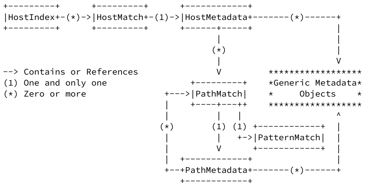
Figure 1: Relationships between CDNI Metadata Objects (Diagram Representation)
