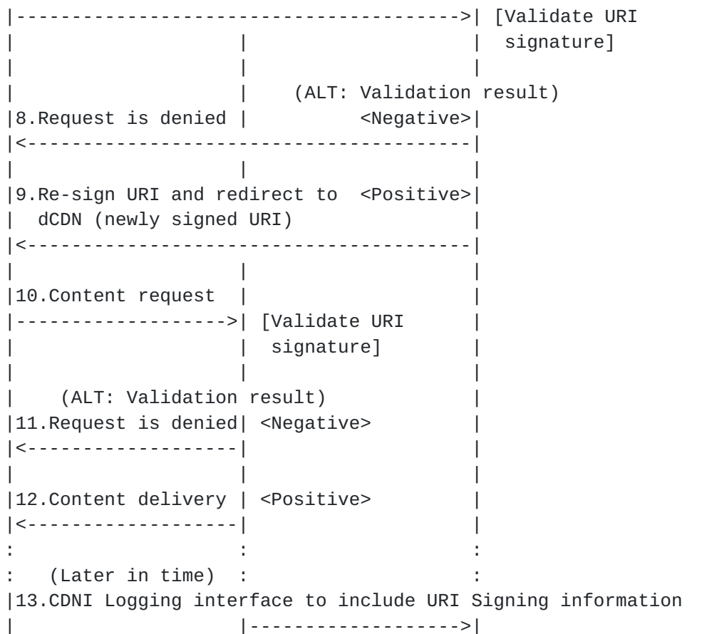
Figure 3: HTTP-based Request Routing with URI Signing
