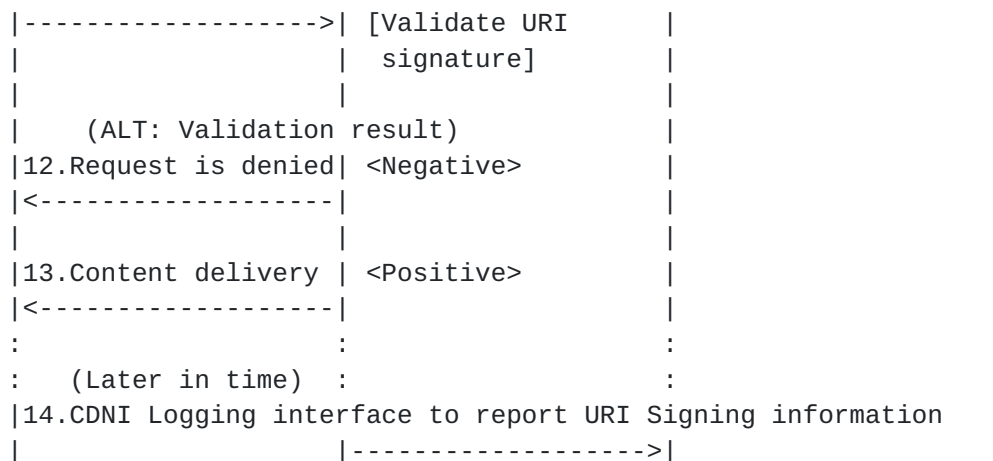
Figure 4: DNS-based Request Routing with URI Signing
