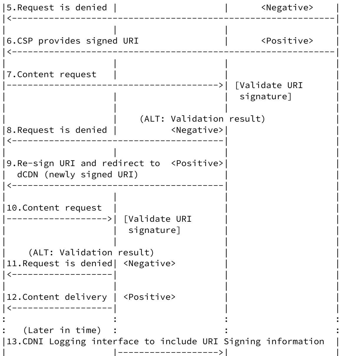
Figure 3: HTTP-based Request Routing with URI Signing
