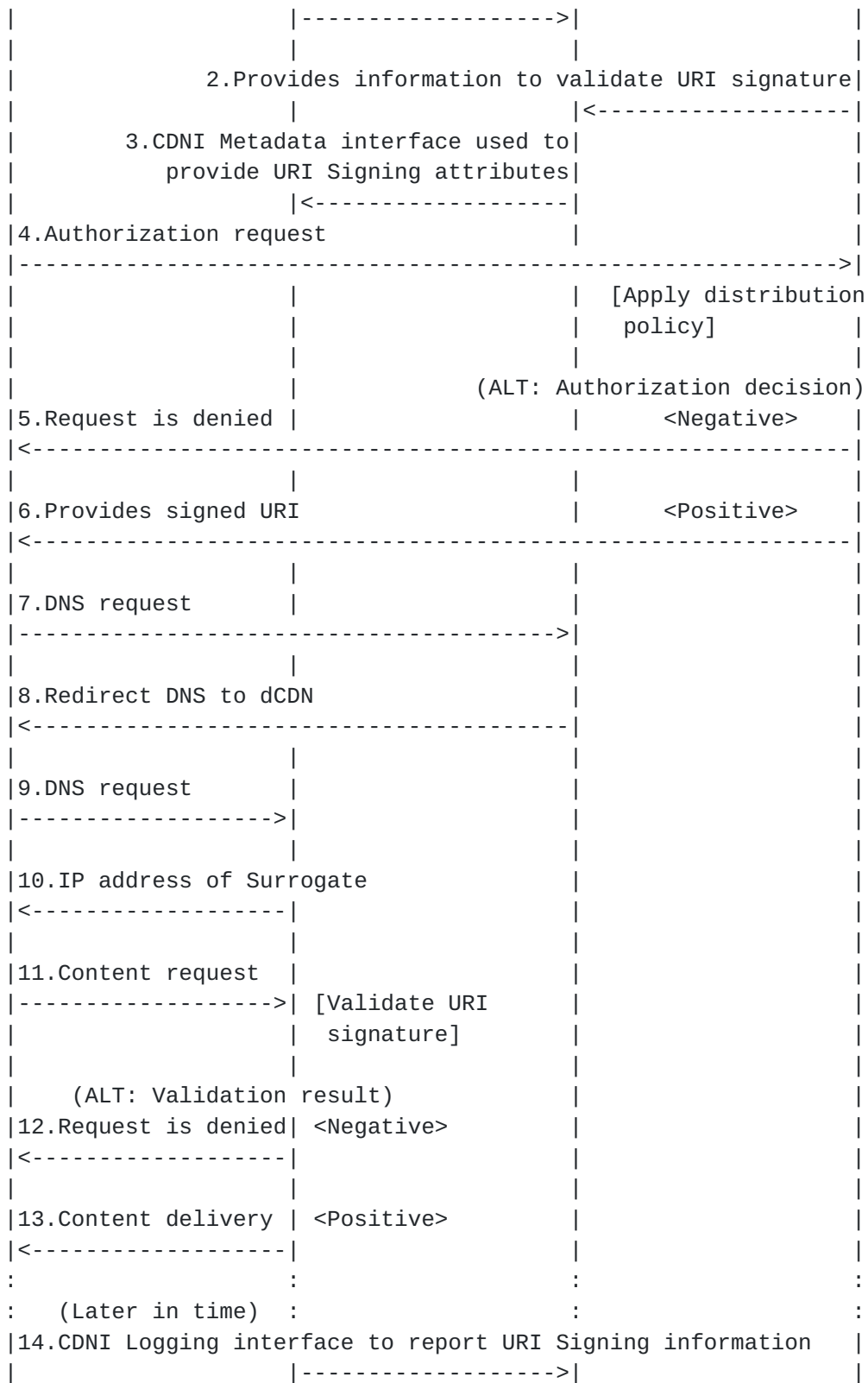
Figure 4: DNS-based Request Routing with URI Signing
