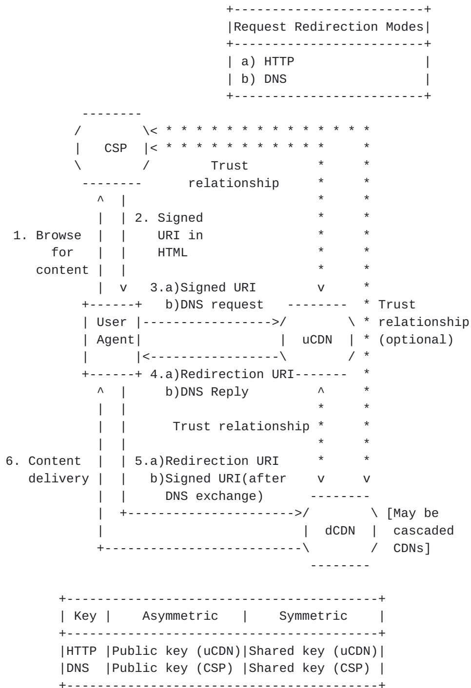
Figure 2: URI Signing in a CDNI Environment
