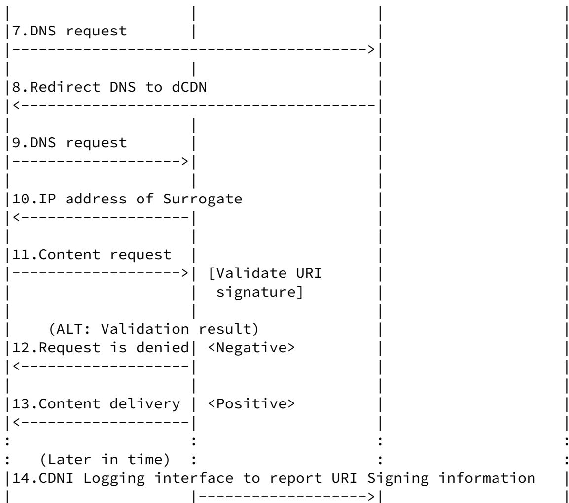
Figure 4: DNS-based Request Routing with URI Signing
