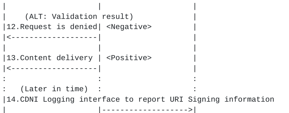
Figure 4: DNS-based Request Routing with URI Signing
