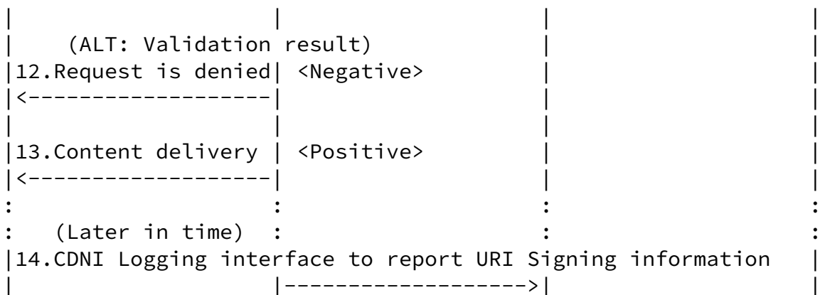
Figure 4: DNS-based Request Routing with URI Signing
