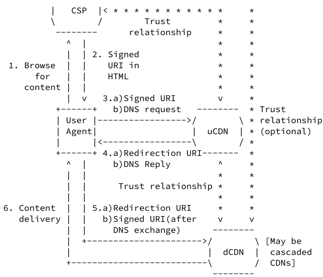
Figure 2: URI Signing in a CDNI Environment
