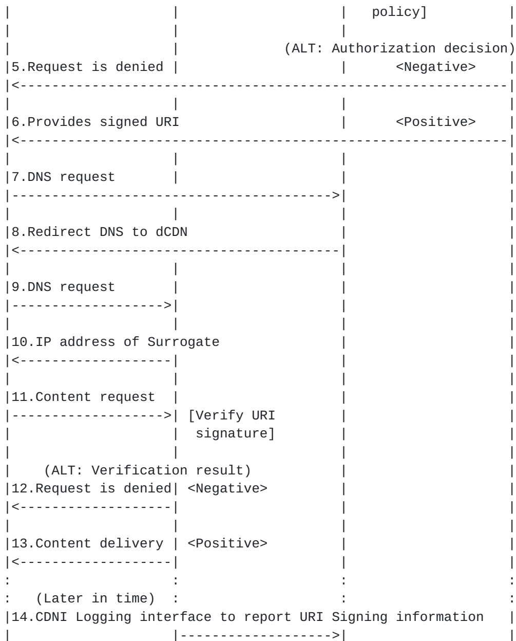
Figure 5: DNS-based Request Routing with URI Signing
