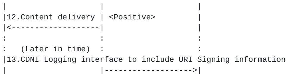
Figure 4: HTTP-based Request Routing with URI Signing
