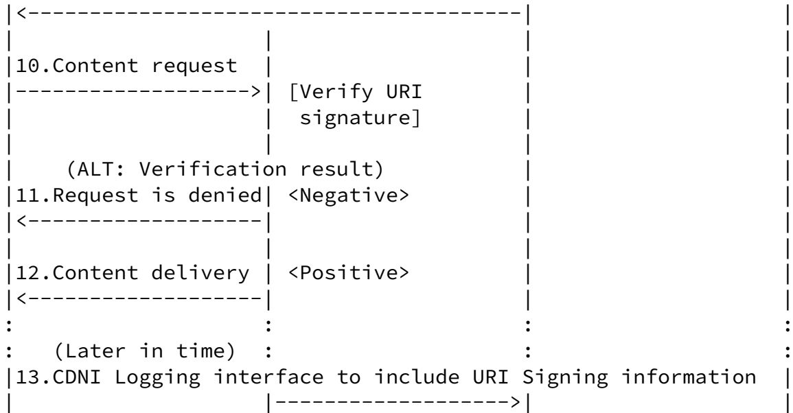
Figure 3: HTTP-based Request Routing with URI Signing
