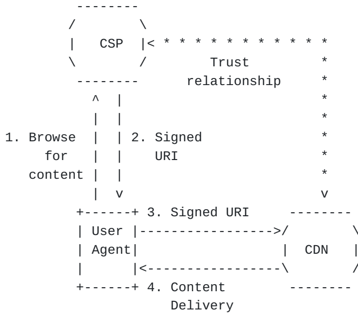
Figure 1: URI Signing in a CDN Environment
