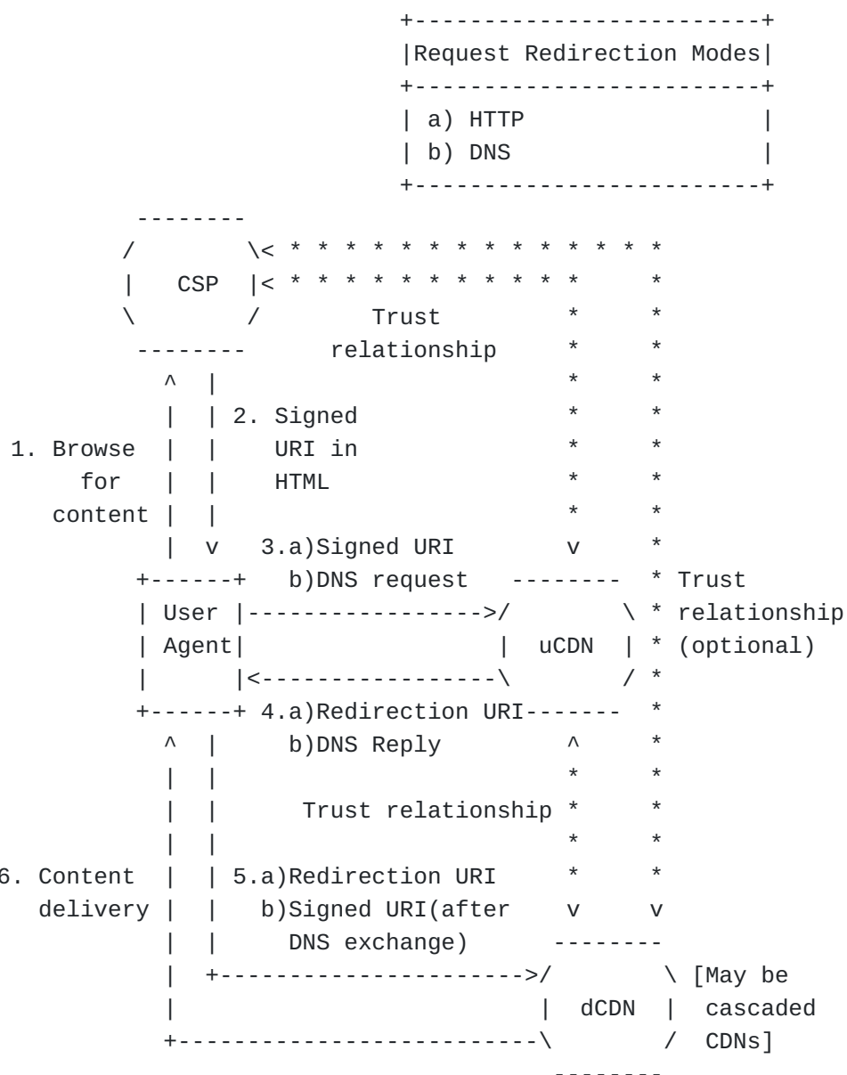
Figure 2: URI Signing in a CDNI Environment
