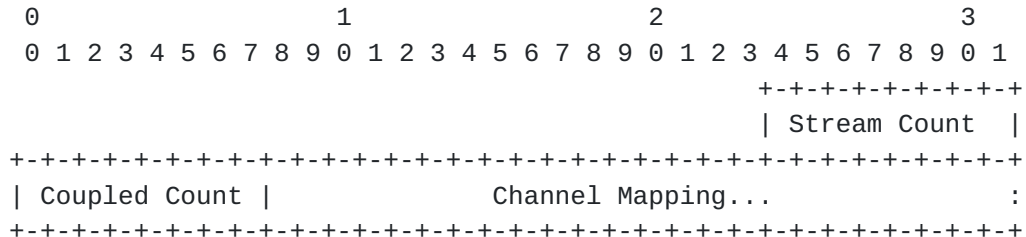
Figure 2: Channel Mapping Table
