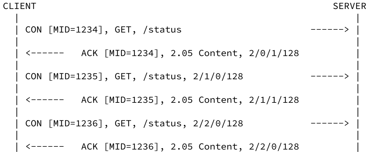
Figure 2: Simple blockwise GET
