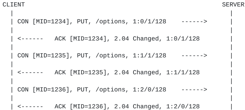
Figure 7: Simple atomic blockwise PUT
