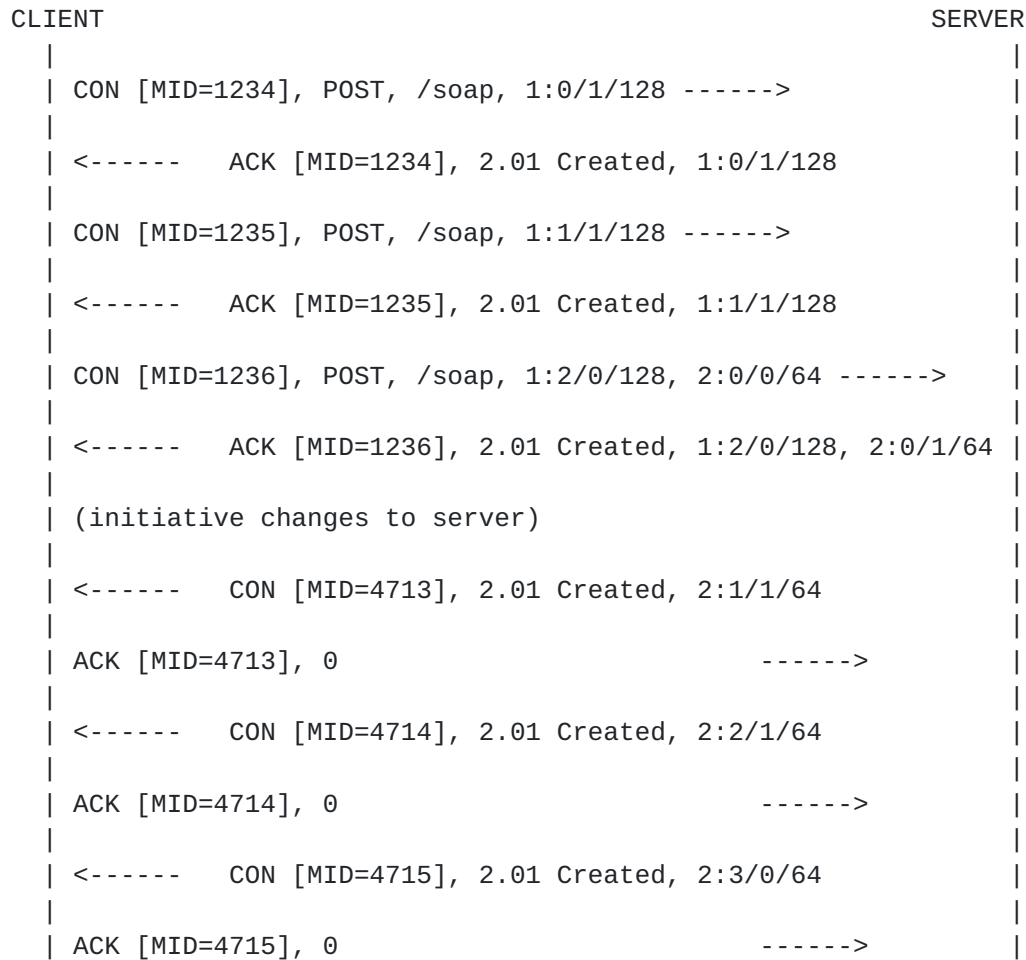
Figure 11: Atomic blockwise POST with separate blockwise response, early negotiation
