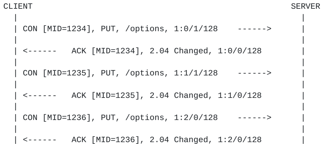
Figure 8: Simple stateless blockwise PUT
