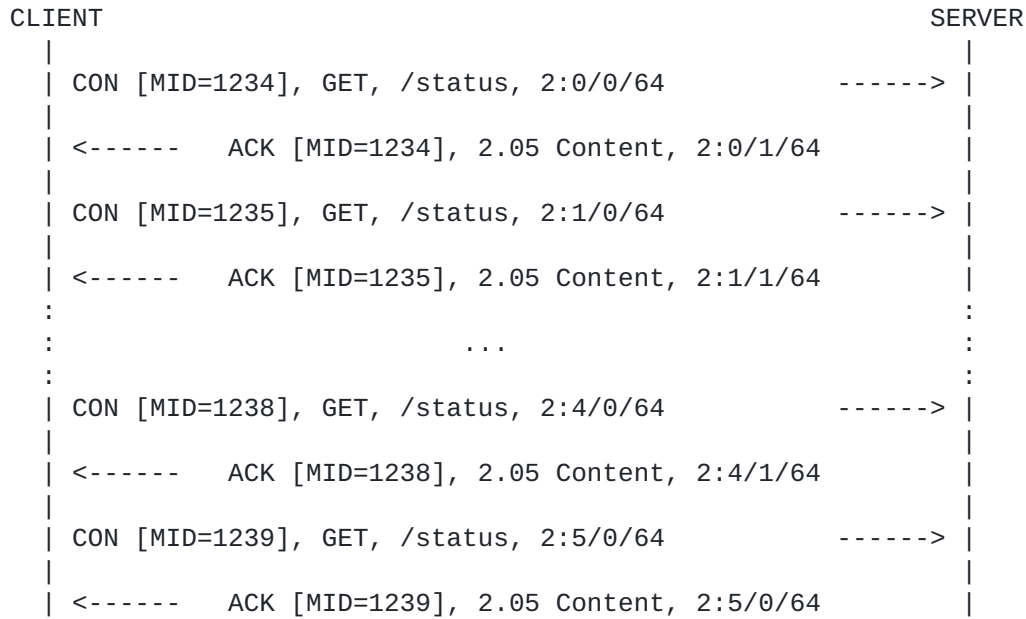
Figure 3: Block-wise GET with early negotiation
