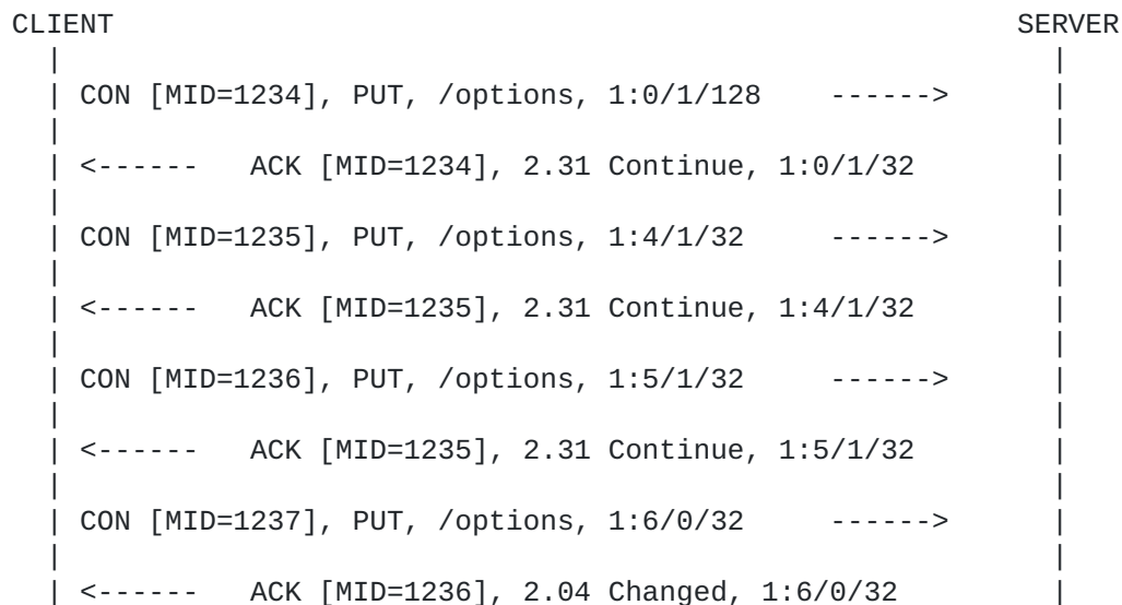
Figure 9: Simple atomic block-wise PUT with negotiation
