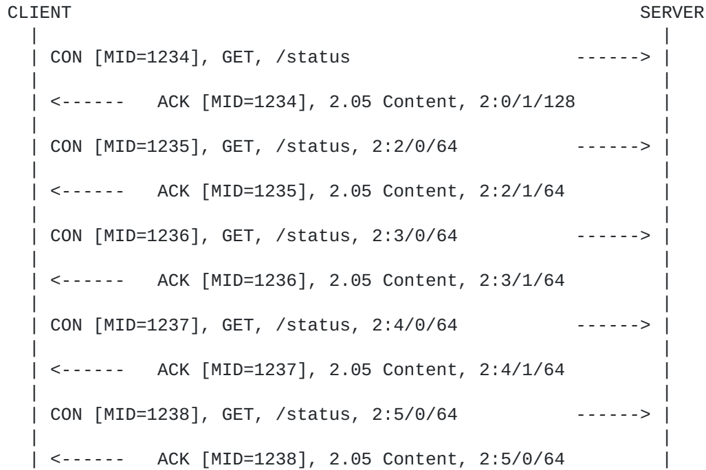
Figure 4: Block-wise GET with late negotiation
