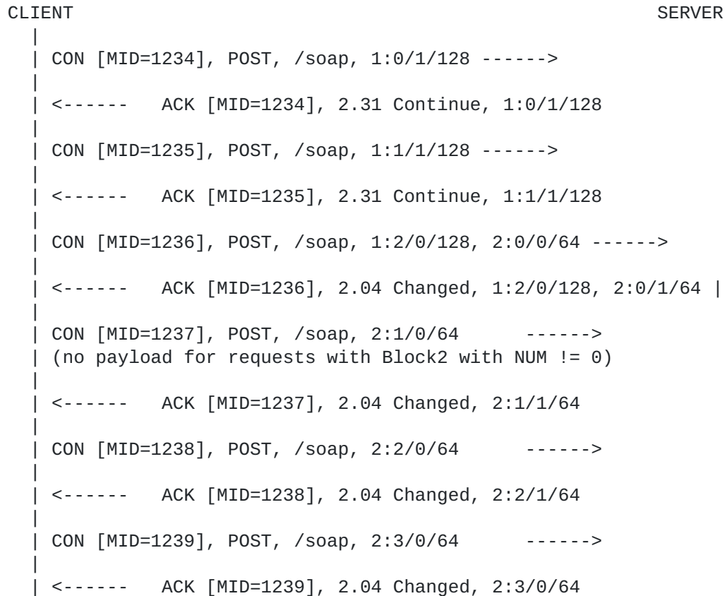
Figure 11: Atomic block-wise POST with block-wise response, early negotiation
