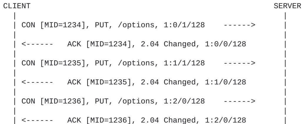
Figure 8: Simple stateless block-wise PUT
