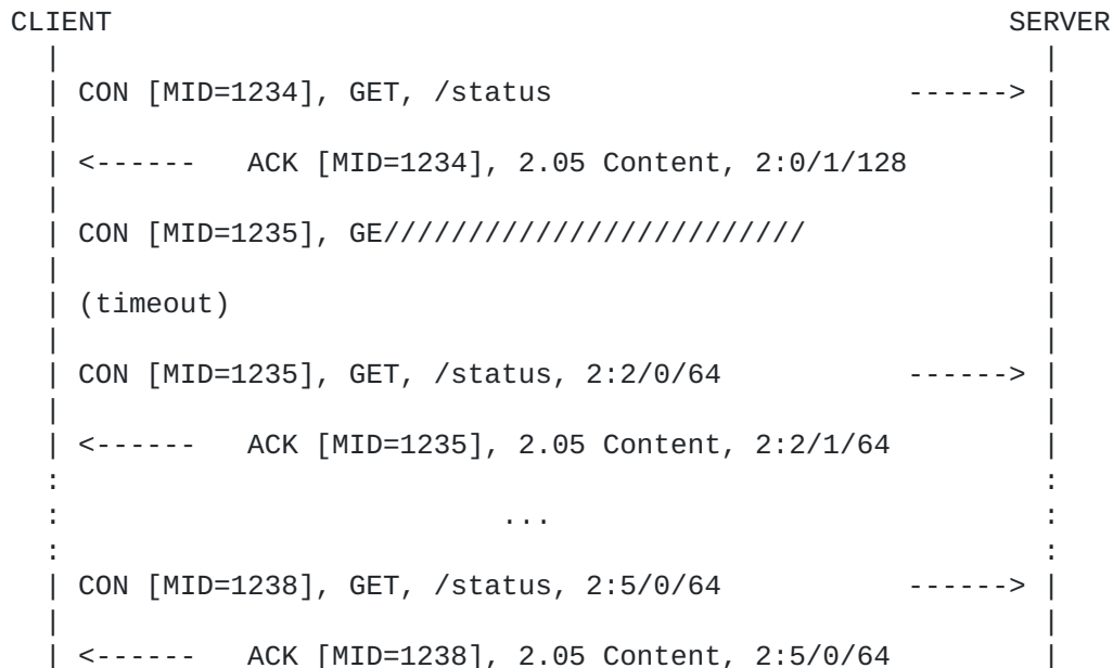
Figure 5: Block-wise GET with late negotiation and lost CON
