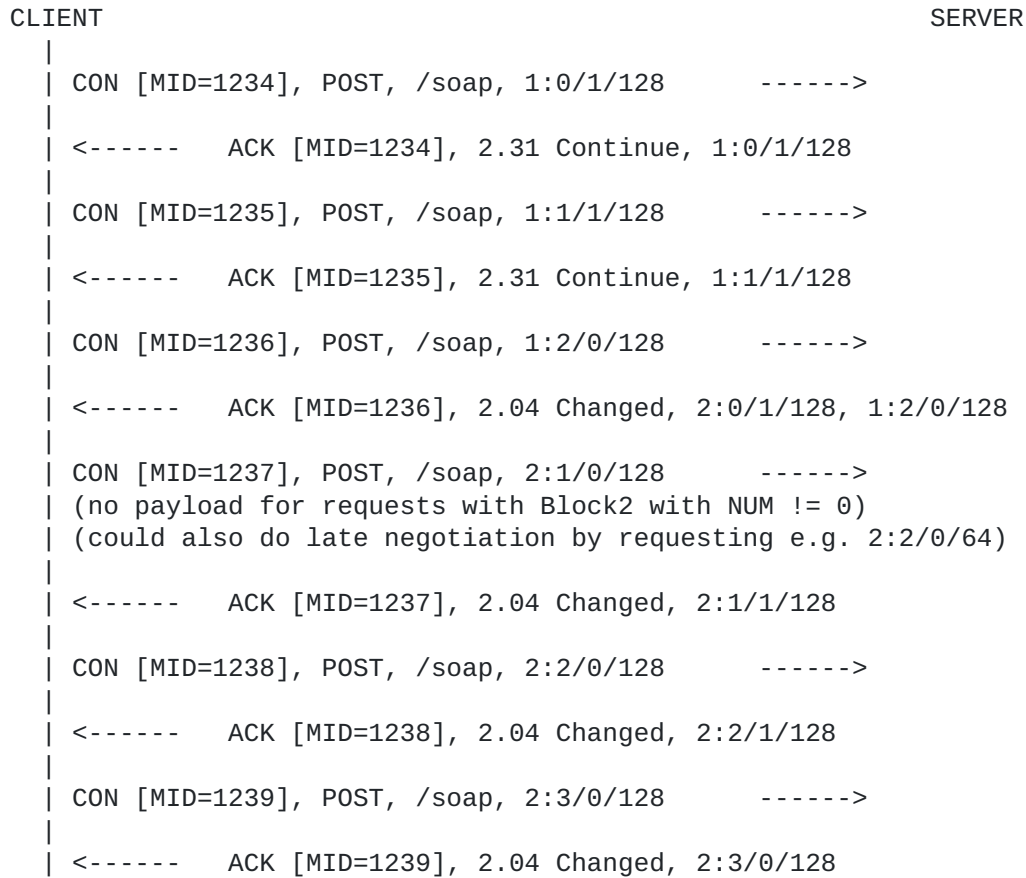
Figure 10: Atomic block-wise POST with block-wise response
