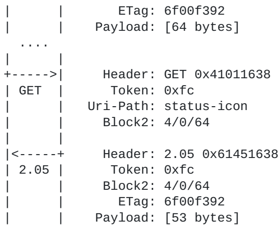
Figure 13: Observe sequence with early negotiation
