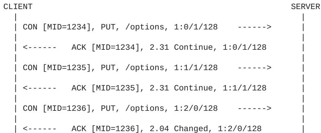
Figure 7: Simple atomic block-wise PUT
