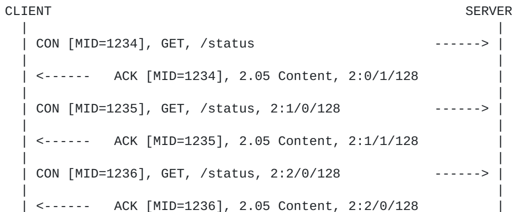
Figure 2: Simple block-wise GET
