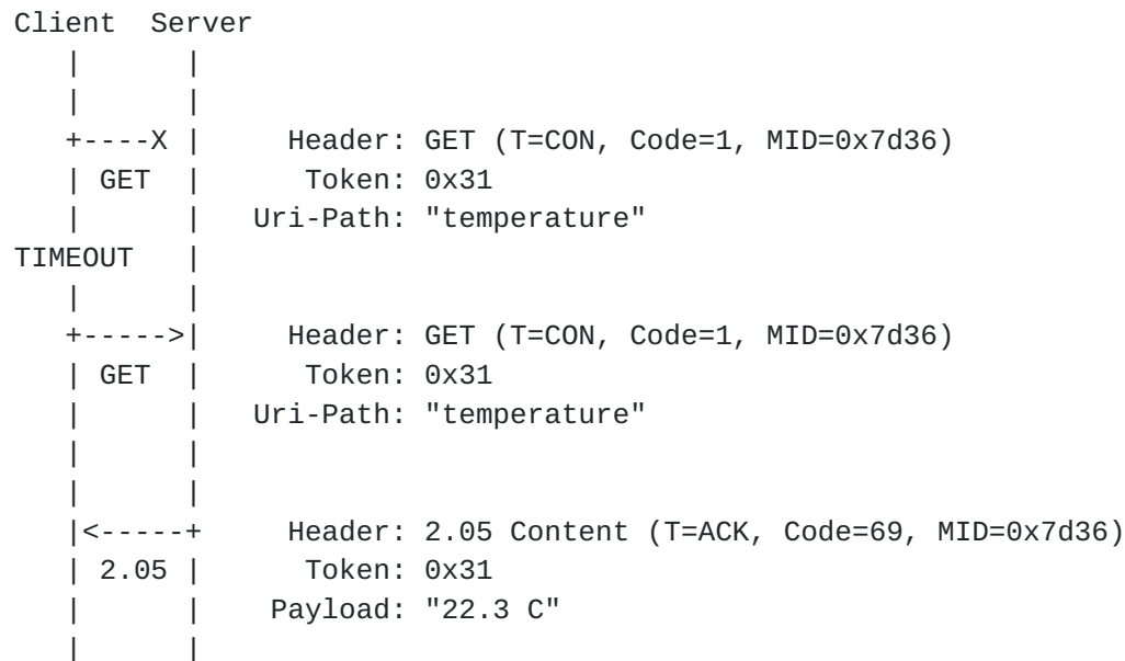
Figure 17: Confirmable request (retransmitted); piggy-backed response
