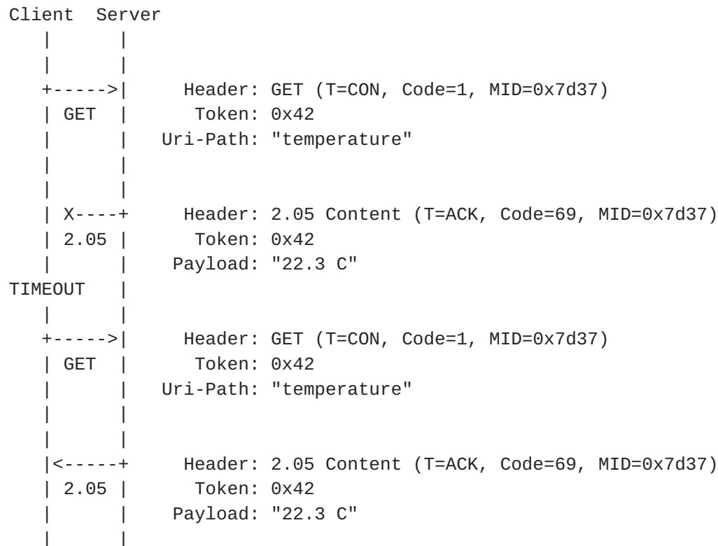
Figure 18: Confirmable request; piggy-backed response (retransmitted)
