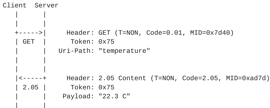
Figure 21: Non-confirmable request; Non-confirmable response
