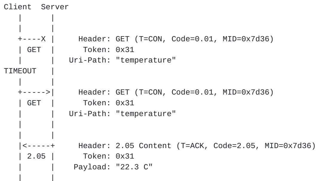
Figure 17: Confirmable request (retransmitted); piggy-backed response
