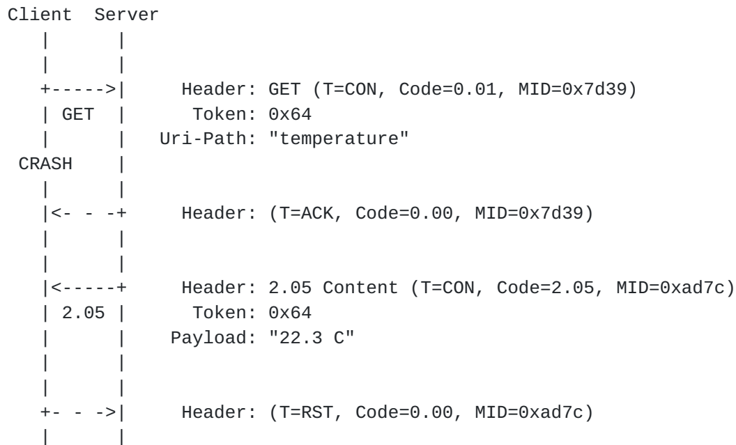
Figure 20: Confirmable request; separate response (unexpected)
