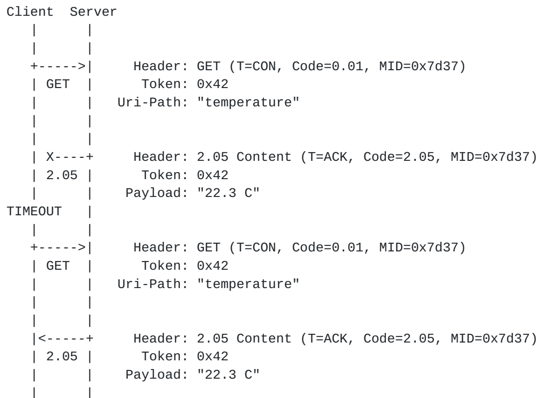
Figure 19: Confirmable request; piggy-backed response (retransmitted)
