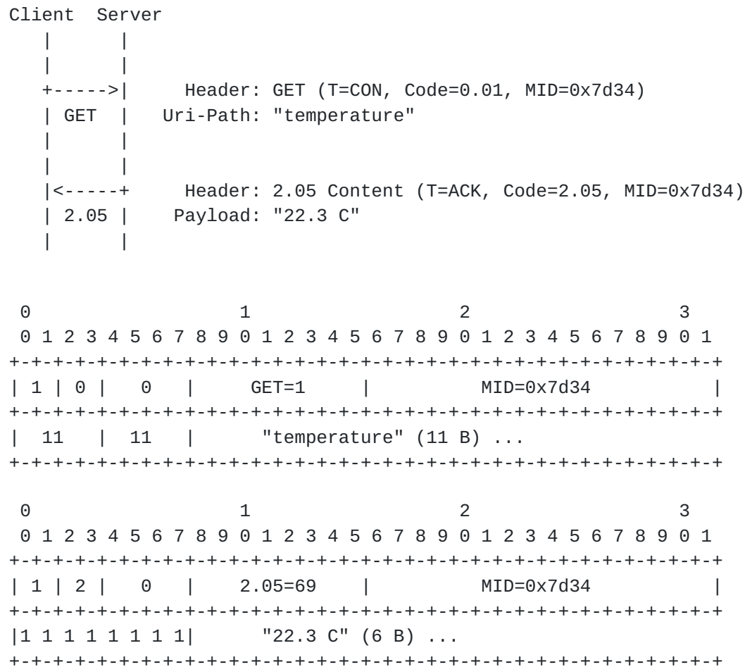
Figure 16: Confirmable request; piggy-backed response
