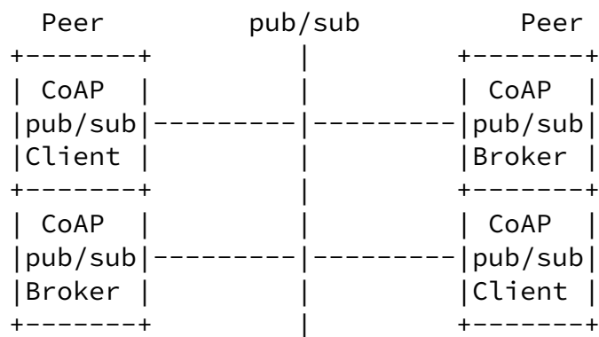
Figure 2: Brokerless pub/sub
