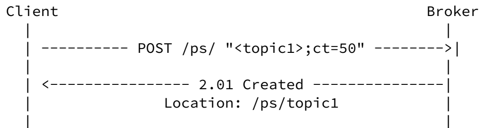
Figure 6: Example of CREATE topic
