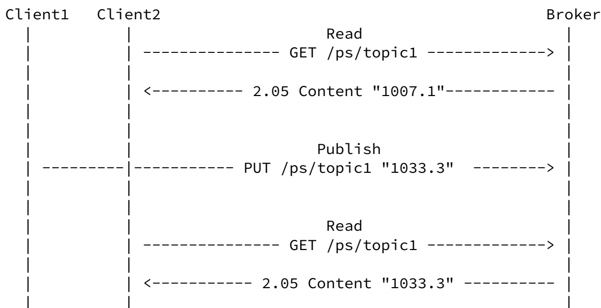
Figure 12: Example of READ
