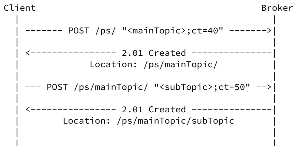
Figure 6: Example of CREATE topic
