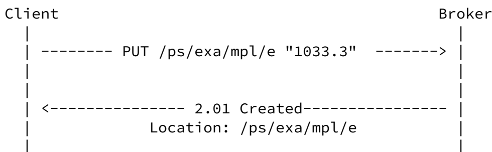
Figure 8: Example of PUBLISH
