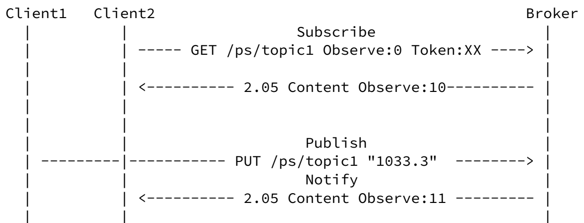
Figure 10: Example of SUBSCRIBE
