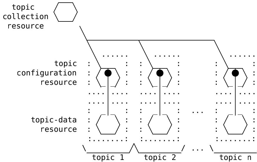
Figure 3: Topic and topic-data resources of a topic
