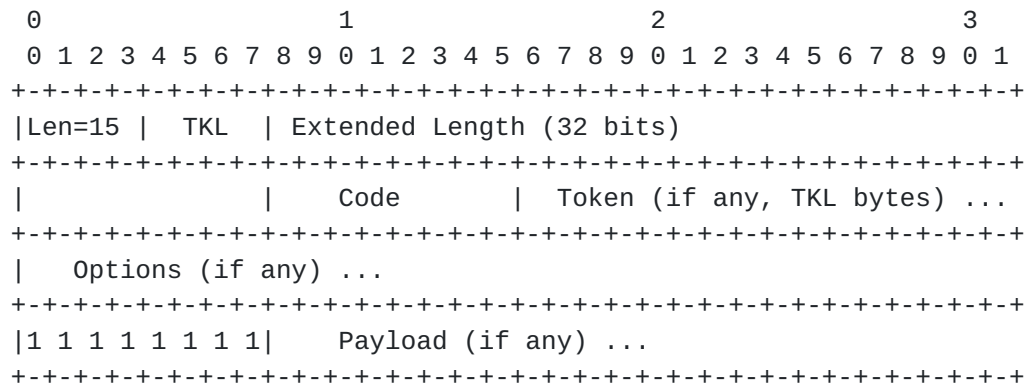
Figure 8: CoAP message format with 32-bit Extended Length field
