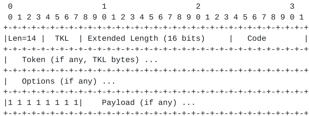
Figure 7: CoAP message format with 16-bit Extended Length field
