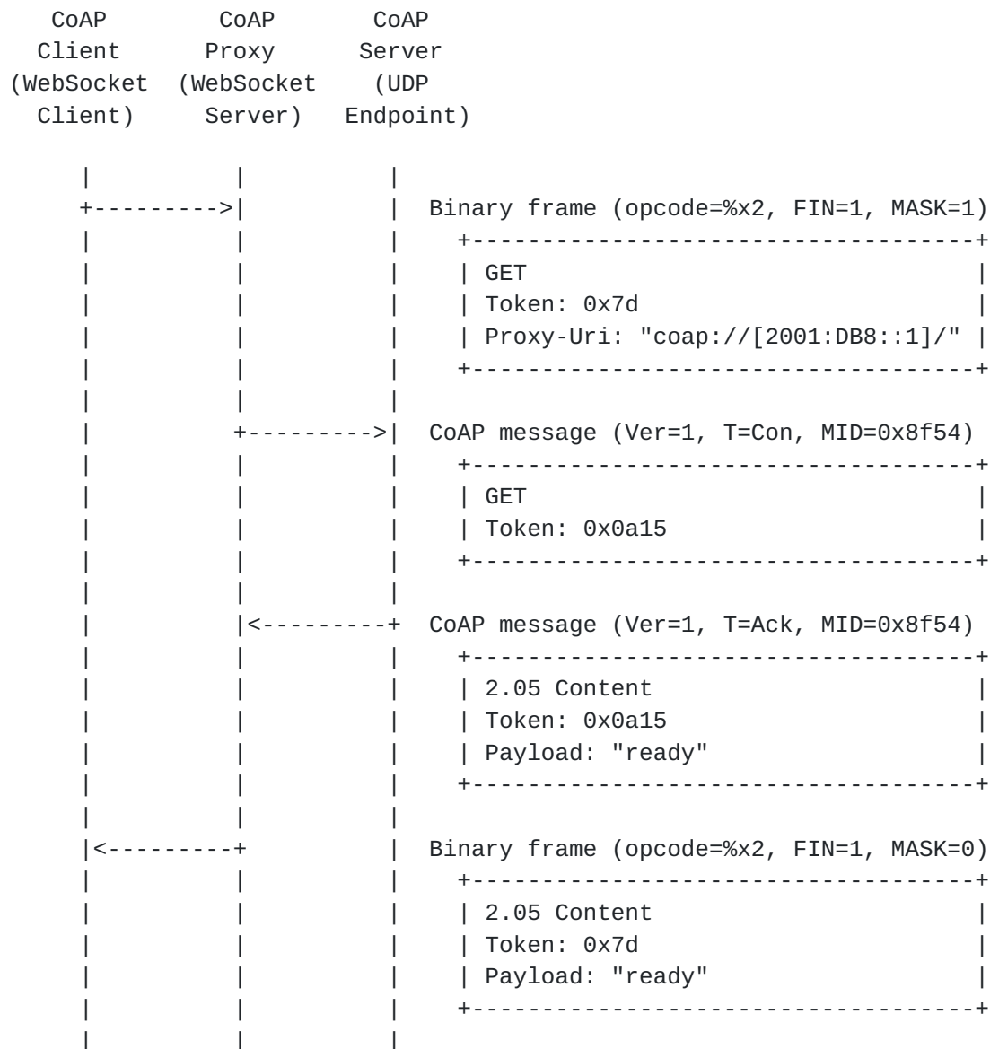
Figure 21: A CoAP client retrieves the representation of a resource identified by a "coap" URI via a WebSockets-enabled CoAP proxy
