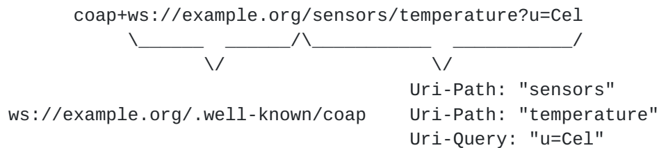
Figure 18: The "coap+ws" URI Scheme
