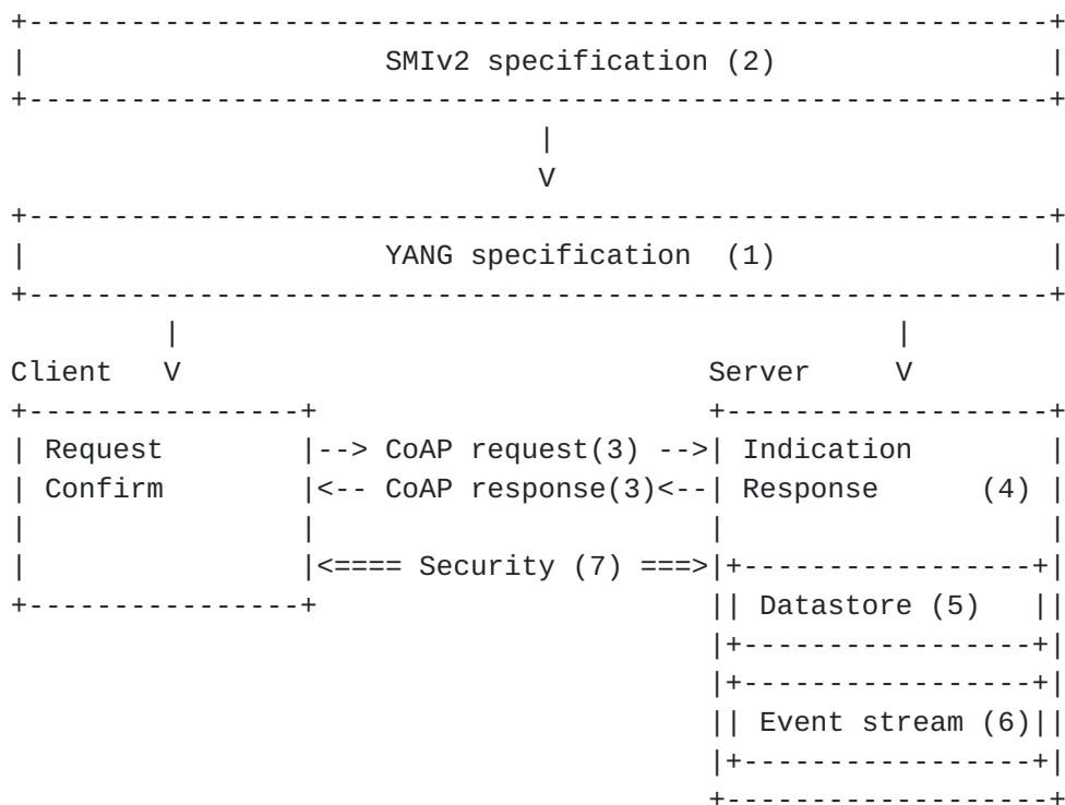
Figure 1: Abstract CoMI architecture
