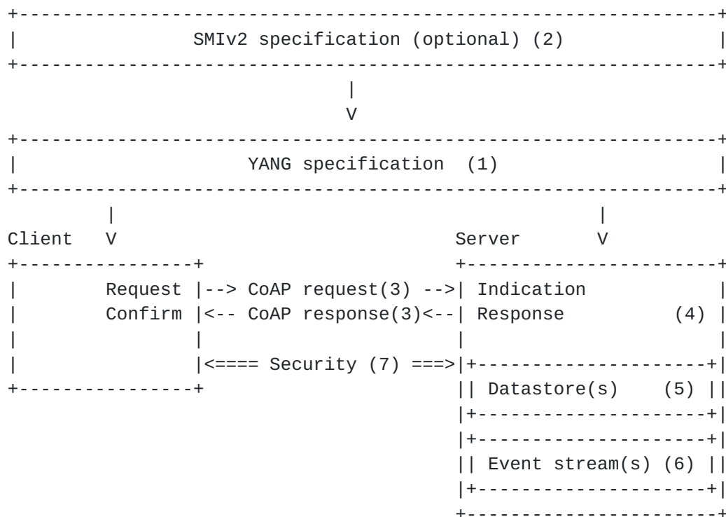
Figure 1: Abstract CORECONF architecture
