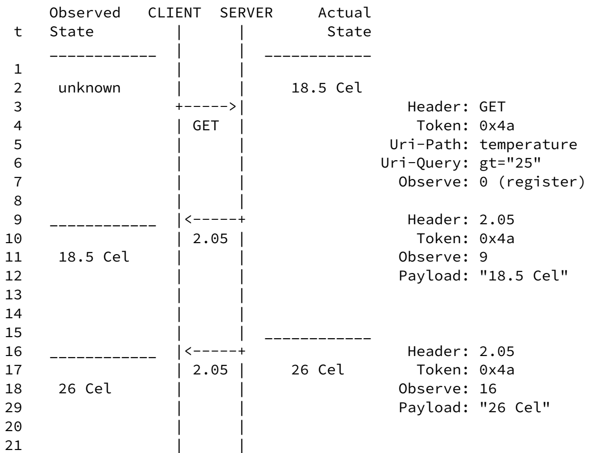
Figure 3: Client Registers and Receives one Notification of the Current State and One of a New State when it passes through the greather than threshold of 25.
