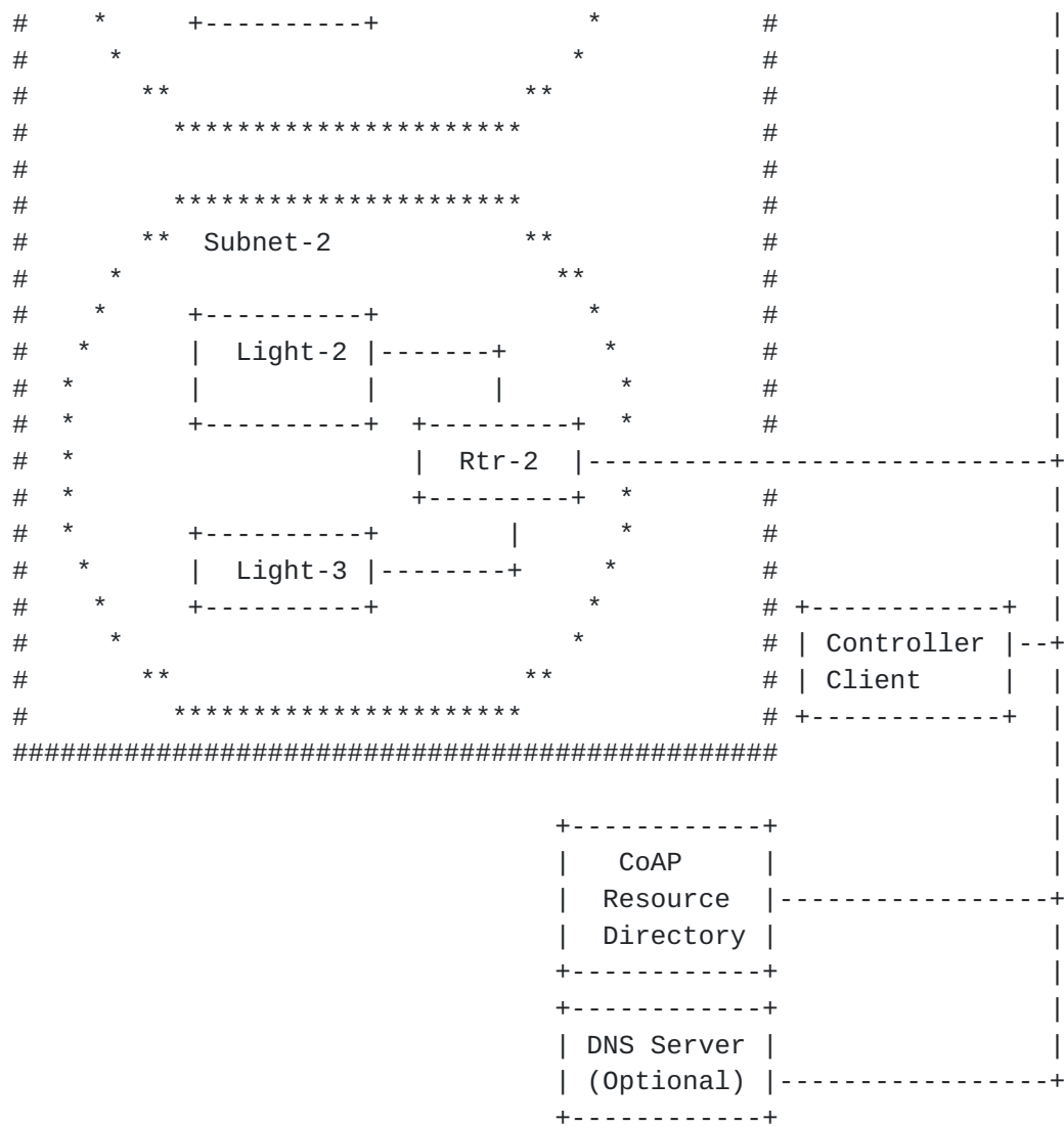
Figure 1: Network Topology of a Large Room (Room-A)
