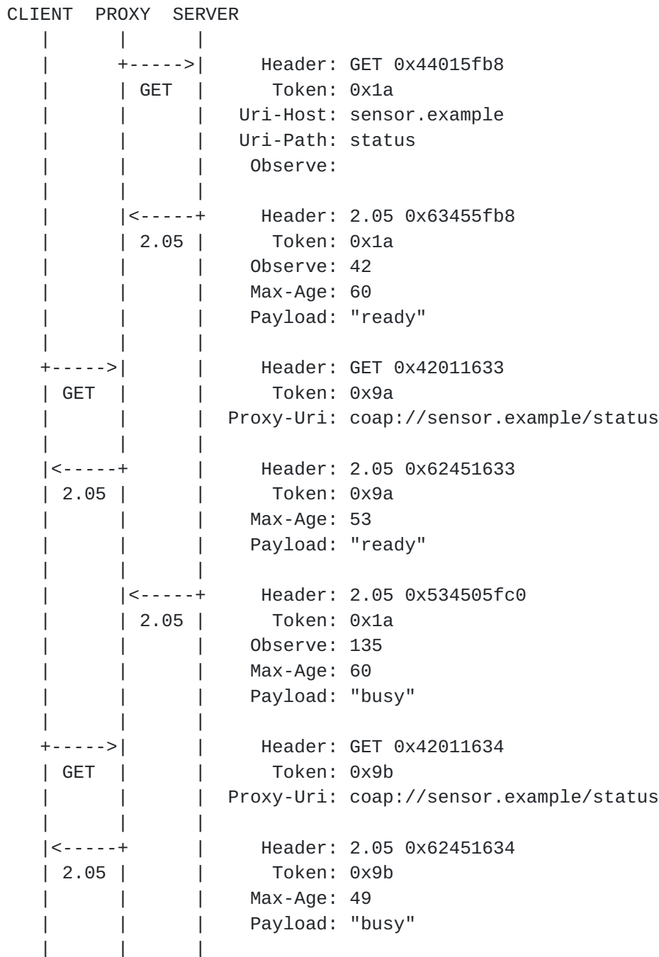
Figure 6: A proxy observes a resource to keep its cache up to date
