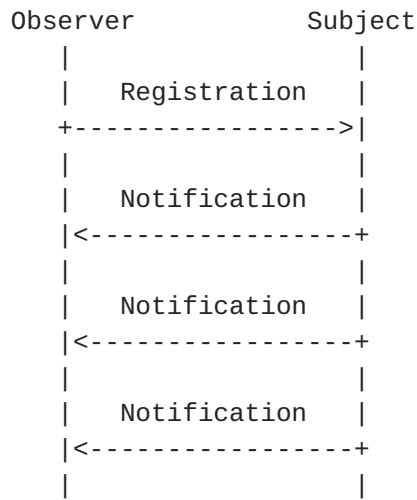
Figure 1: Observer Design Pattern
