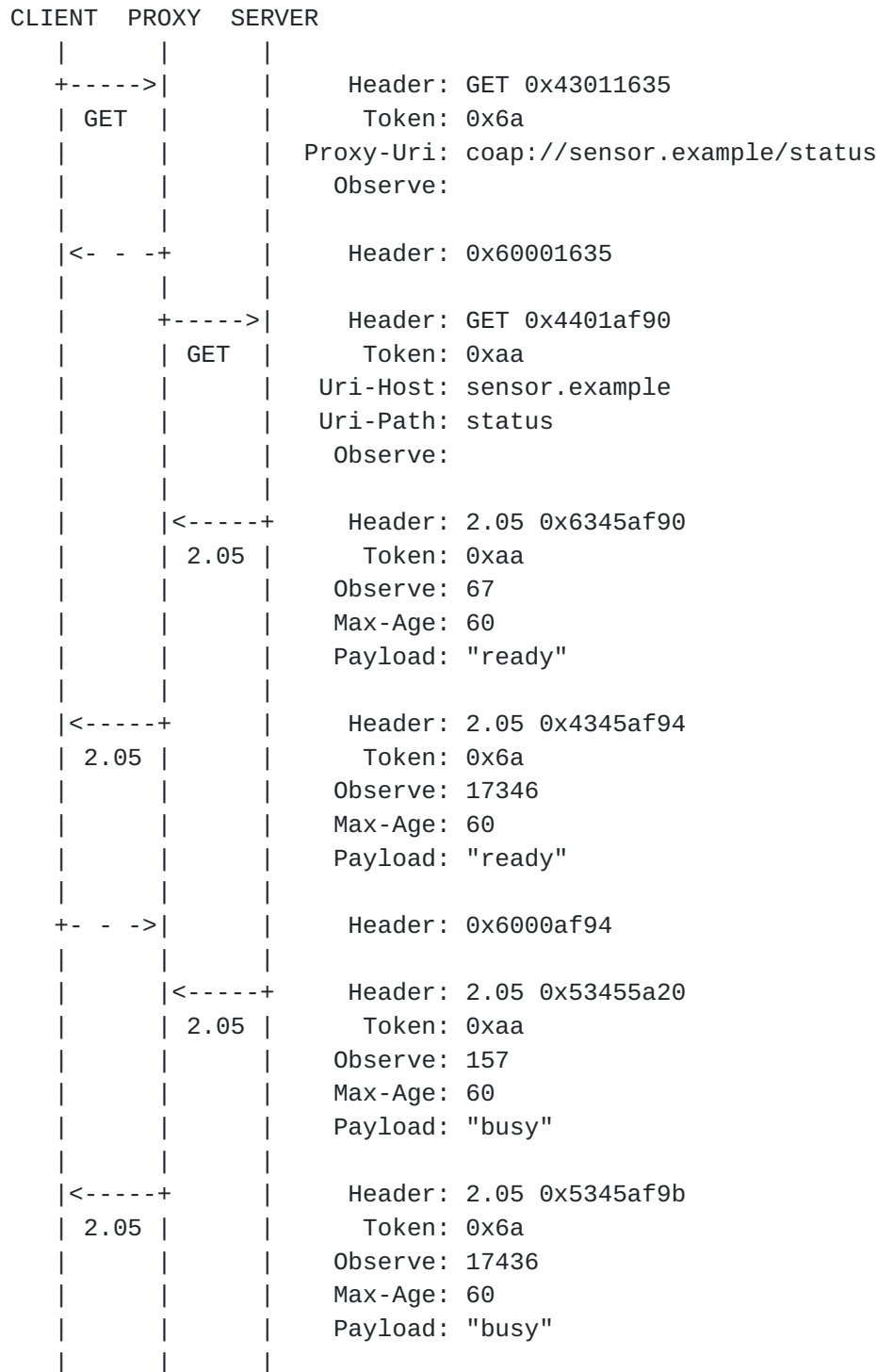
Figure 7: A client observes a resource through a proxy
