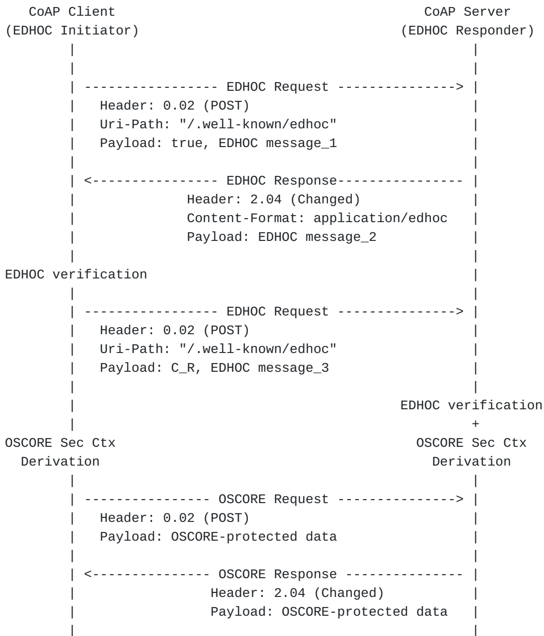
Figure 1: EDHOC and OSCORE run sequentially
