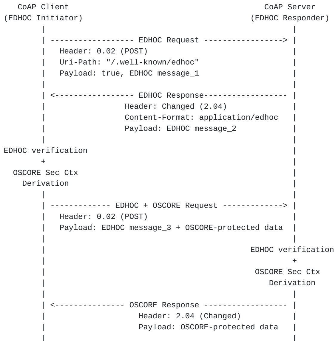
Figure 2: EDHOC and OSCORE combined
