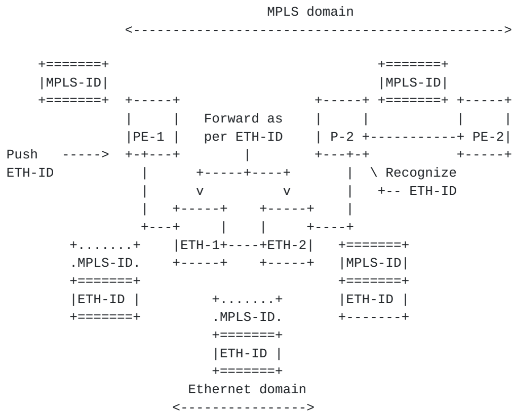
Figure 9: MPLS nodes interconnected by an Ethernet domain
