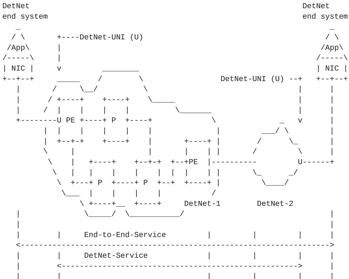
Figure 2: DetNet Service Reference Model (multi-domain)
