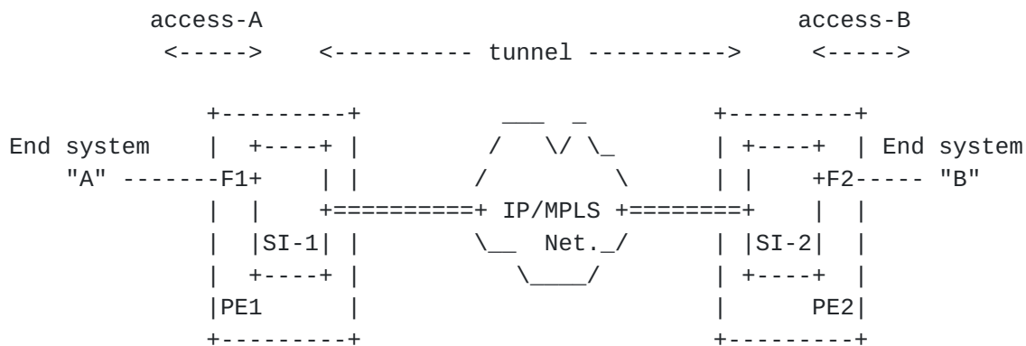
Figure 5: DetNet network reference model
