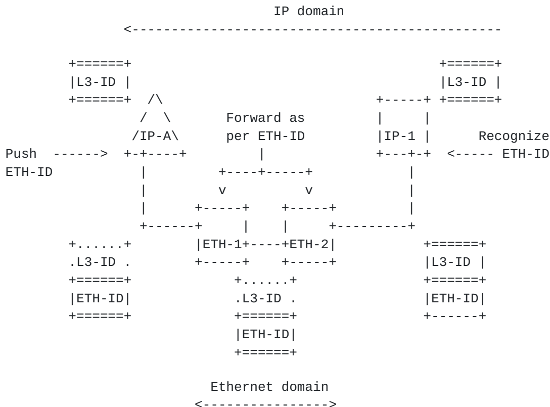
Figure 8: IP nodes interconnected by an Ethernet domain
