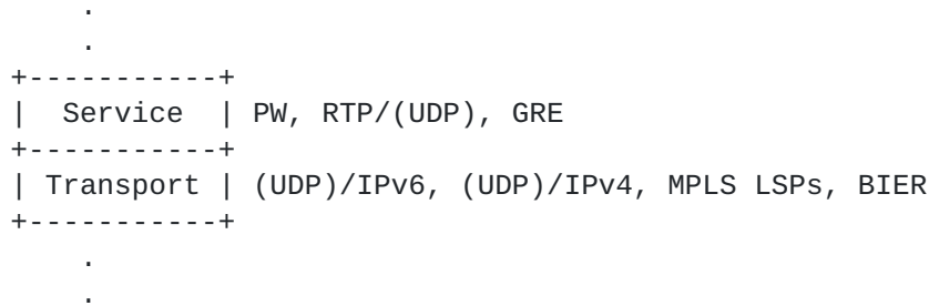
Figure 4: DetNet adaptation to data plane
