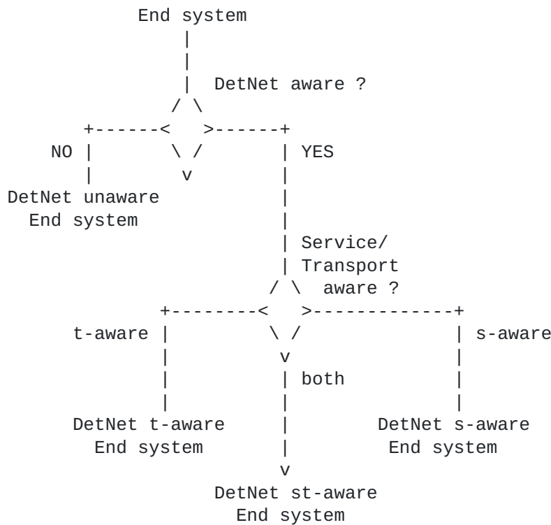
Figure 6: Grouping of end systems
