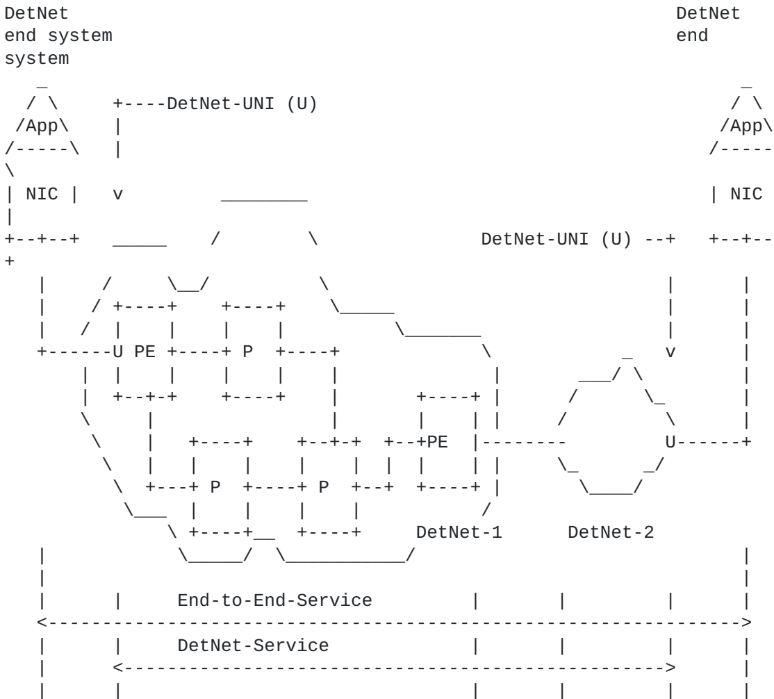
Figure 5: DetNet Service Reference Model (multi-domain)
