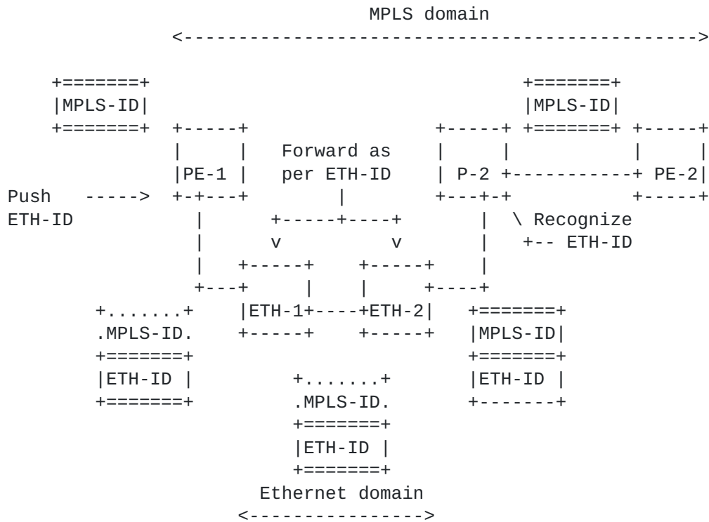
Figure 11: MPLS nodes interconnected by an Ethernet domain
