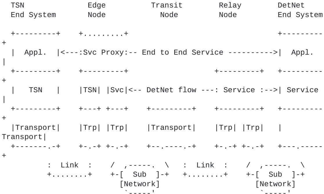
Figure 3: A Simple DetNet Enabled Network
